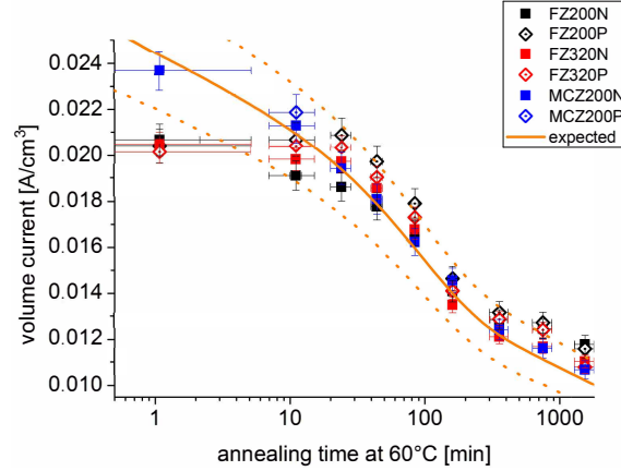
Figure 12. Volume current density as a function of annealing time at +60^\circ\text{C} shown for diodes irradiated with neutrons to \phi_{\text{eq}} = 4 \times 10^{14} \text{ cm}^{-2} . For comparison, the current density versus annealing time expected for this fluence based on a parameterization and parameters obtained by previous fits to data [1, 3] is depicted by a solid line. The corresponding uncertainty, shown as dashed lines, is due to the uncertainty in the fluence, estimated to be about 10%.
