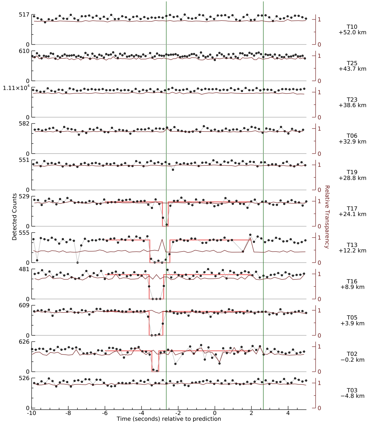
Figure 8. Observations from 2017-07-17 occultation, part 1. The figure shows the lightcurves from the northern half of the data collected by the mobile stations. Each sub-plot is labeled on the right with the team number and the cross-track offset. The team numbers are cross-referenced with Table 4. The plots indicate the signal level from each station – higher numbers indicate higher signal levels. The
