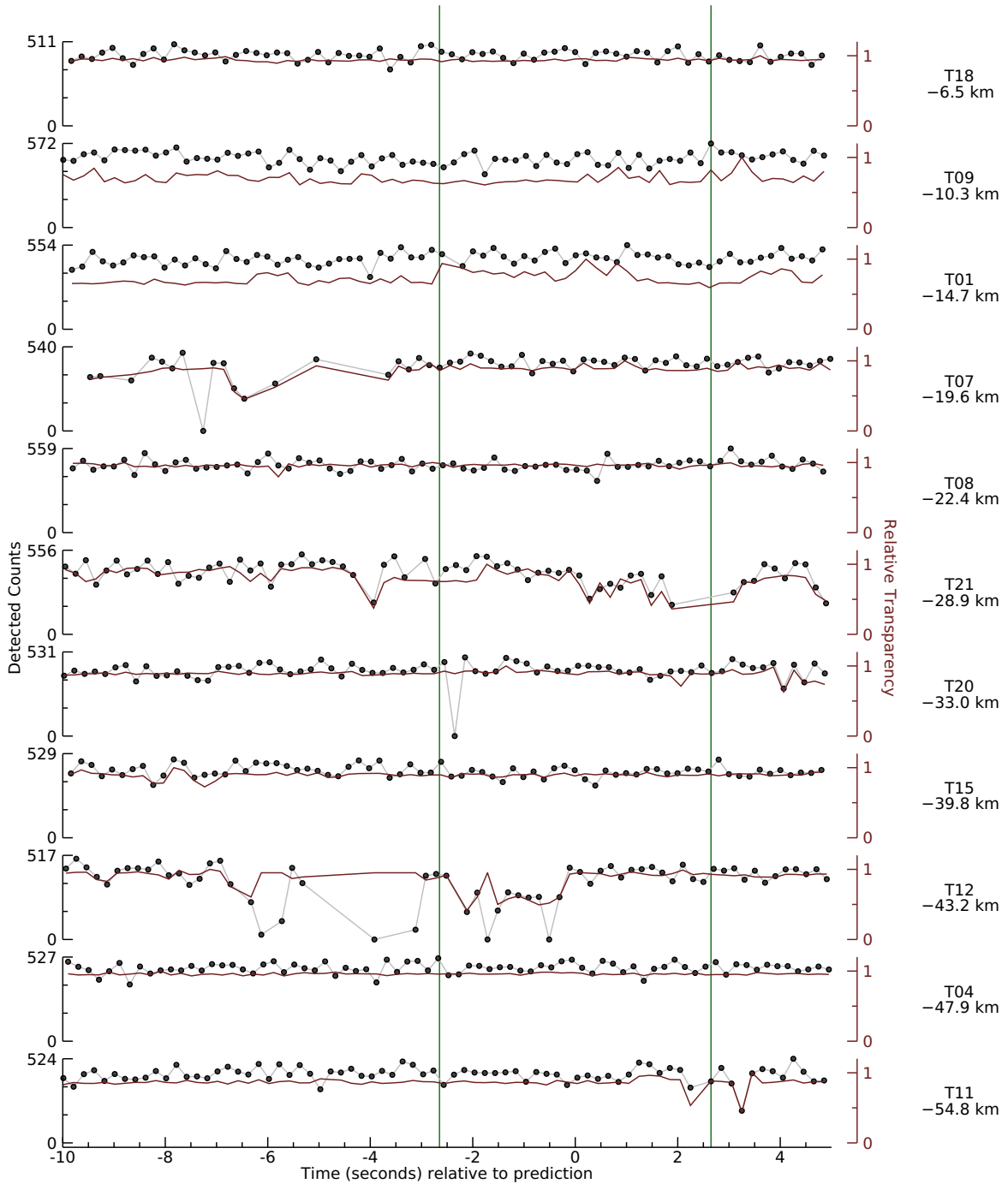
Figure 9. Observations from 2017-07-17 occultation, part 2. The figure shows the lightcurves from the southern half of the data collected by the mobile stations. Each sub-plot is labeled on the right with the team number and the cross-track offset. The team numbers are cross-referenced with Table 4. The plots indicate the signal level from each station – higher numbers indicate higher signal levels. The green vertical lines indicate the predicted 3\text{-}\sigma uncertainty limits for the event. The second (brown) curve plotted is an estimate of the relative transparency. An electronic copy of the data in this figure is provided.
