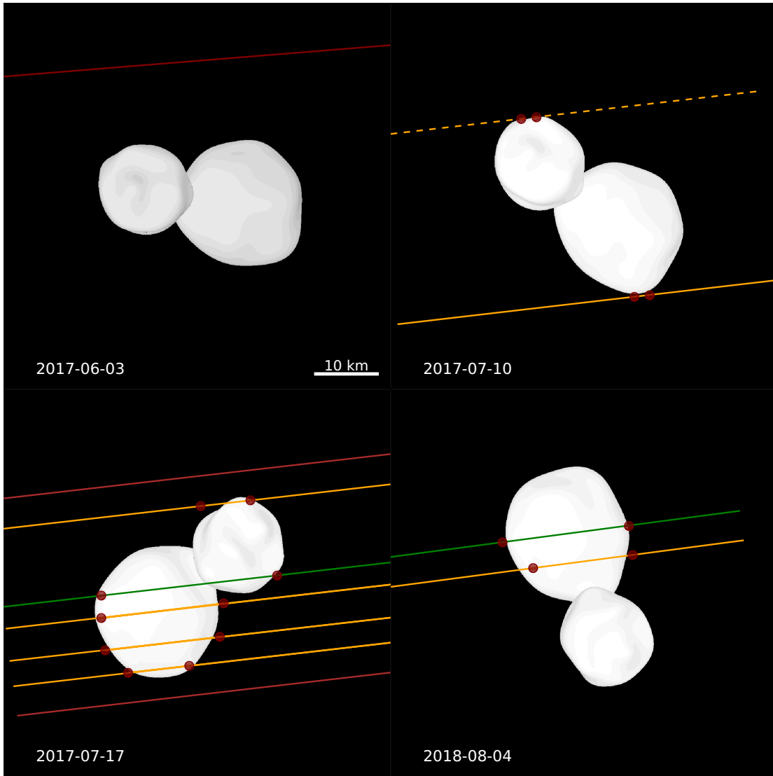
Figure 13. Comparison of shape model with occultation data. The projected shape and orientation of Arrokoth is compared to the occultation data for all four events in a J2000 sky-plane view. Red lines indicate observations that did not record an occultation. Green and yellow lines are those that did. The red dots denote where the star either disappeared or reappeared. The dashed yellow line for 2017-07-10 is an alternate but less favored option.
