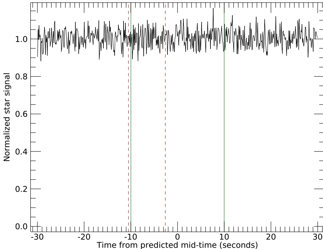
Figure 4. SAAO observations for the 2017-06-03 occultation. The figure shows the lightcurve obtained from SAAO. We see no event in the data. The solid green lines indicate \pm 3\sigma relative to the “may25a” prediction. The dashed purple lines indicate \pm 3\sigma relative to the final “ey7” post-diction. The cross track offset based on “ey7” is 17.4\pm 4.0 km. See Section 7.7 for an explanation of the terms “may25a”, and “ey7”. An electronic copy of the data in this figure is provided.
