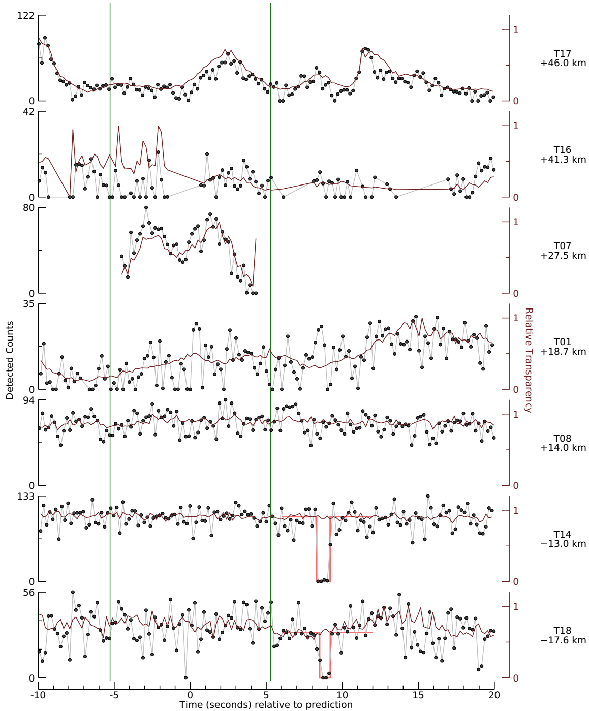
Figure 12. Observations from 2018 Aug 04 occultation. The figure shows the lightcurves collected by the mobile stations. Each sub-plot is labeled on the right with the team number and the cross-track offset. The team numbers may be cross-referenced with Table 6. The plots indicate the signal level from each station – higher numbers indicate higher signal levels. The green vertical lines indicate the predicted 3\sigma uncertainty limits for the event. The second (brown) curve plotted is an estimate of the relative transparency. Two of these curves show an overlain solid-body model used to extract occultation timings. An electronic copy of the data in this figure is provided.
