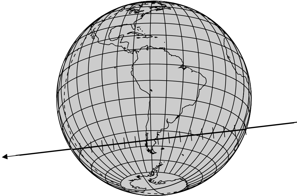
Figure 7. Global view of 2017-07-17 occultation prediction. The figure shows the Earth as seen from Arrokoth at the time of geocentric closest approach. The Sun is below the horizon in the regions shaded gray (the entire globe). The dashed line shows where the Sun is at -12^\circ altitude. The solid line indicates the predicted ground-track with the width drawn to scale for a 30 km diameter object. The arrowhead indicates the direction of motion and the ticks are spaced at 30 second intervals from 03:46:00 to 03:53:30 UT. Shadow velocity was 23.5 \text{ km s}^{-1} . A 46% illuminated Moon was 105^\circ from the target at the time of the event.
