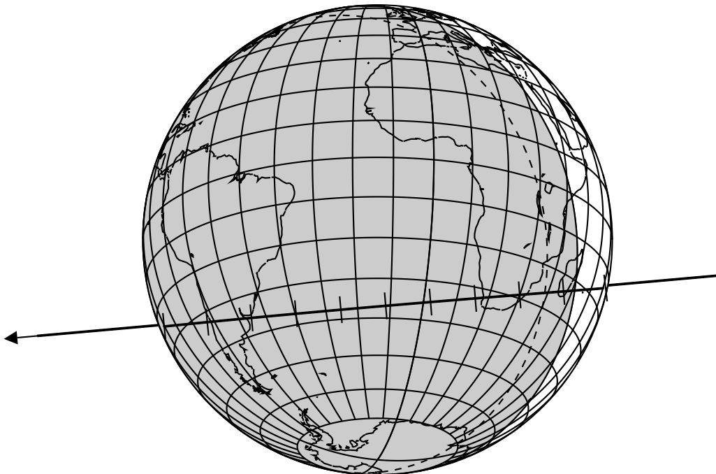
Figure 1. Global view of 2017-06-03 occultation prediction. The figure shows the Earth as seen from Arrokoth at the time of geocentric closest approach. The Sun is below the horizon in the regions shaded gray. The dashed line indicates -12^\circ Sun altitude. The solid line indicates the predicted ground-track with the width drawn to scale for a 30 km diameter object. The arrowhead indicates the direction of motion and the ticks are spaced at one minute intervals from 03:07 to 03:17 UT. Shadow velocity was 20.0\ \text{km s}^{-1} . A 66% illuminated Moon was 103^\circ away from the target at the time of the event but was below the horizon in Africa.
