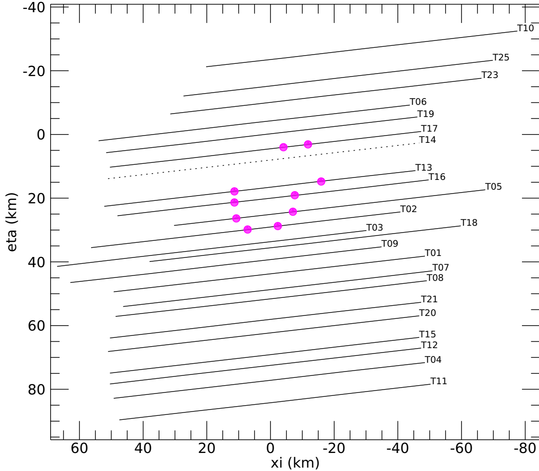
Figure 10. Geometry plot of the 2017-07-17 occultation. Each line shows a track of the topocentric position of Arrokoth relative to the star for 30 seconds around the time of the event and is labeled with the team number. The stagger between curves is due to the variation on longitude of the observing sites. The magenta dots indicate the interval where we observed the occultations. The one dotted curve did not yield timing information because of mis-pointing at the time of the event. The team numbers may be cross-referenced with Table 4.
