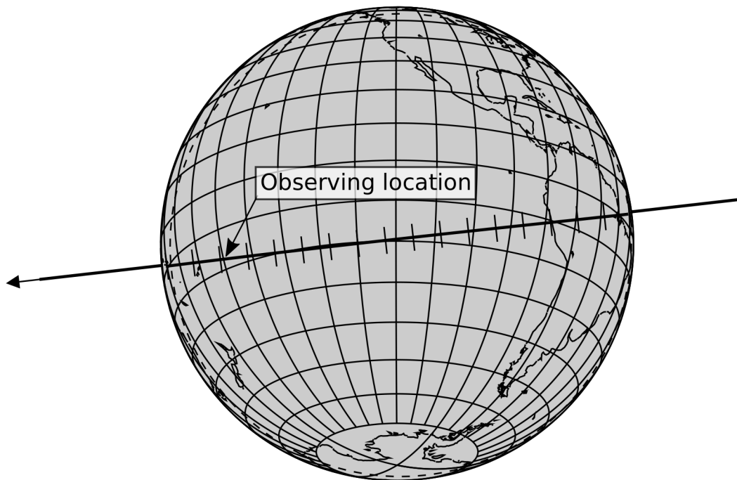
Figure 5. Global view of 2017-07-10 occultation prediction. The figure shows the Earth as seen from Arrokoth at the time of geocentric closest approach. The Sun is below the horizon in the regions shaded gray (the entire globe). The dashed line shows where the Sun is at -12^\circ altitude. The solid line indicates the predicted ground-track with the width drawn to scale for a 30 km diameter object. The arrowhead indicates the direction of motion and the ticks are spaced at 30 second intervals from 07:41:30 to 07:50:00 UT. Shadow velocity was 25.0 \text{ km s}^{-1} . A 99% illuminated Moon was 17^\circ away from the target at the time of the event.
