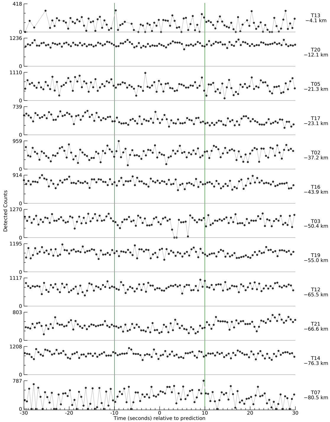
Figure 3. Observations from 2017-06-03 occultation, part 2. The figure shows the lightcurves from the southern half of the data collected by the mobile stations. Each sub-plot is labeled on the right with the team number and the cross-track offset. The team numbers are cross-referenced with Table 2. The plots indicate the signal level from each station – higher numbers indicate higher signal levels. The green vertical lines indicate the predicted 3\text{-}\sigma uncertainty limits for the event. An electronic copy of the data in this figure is provided.
