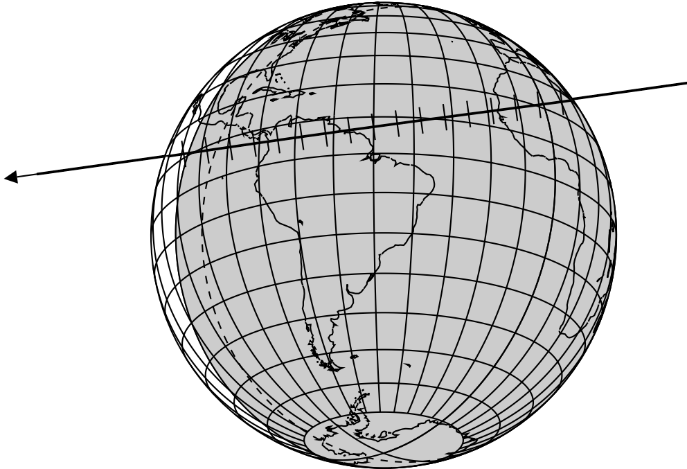
Figure 11. Global view of 2018-08-04 occultation prediction. The figure shows the Earth as seen from Arrokoth at the time of geocentric closest approach. The Sun is below the horizon in the regions shaded gray. The dashed line shows where Sun is at -12^\circ altitude. The solid line indicates the predicted ground-track with the width drawn to scale for a 30 km diameter object. The arrowhead indicates the direction of motion and the ticks are spaced at 30 second intervals from 01:20:00 to 01:28:00 UT. Shadow velocity was 21.4 \text{ km s}^{-1} . A 58% illuminated Moon was 108^\circ away from the target at the time of the event.
