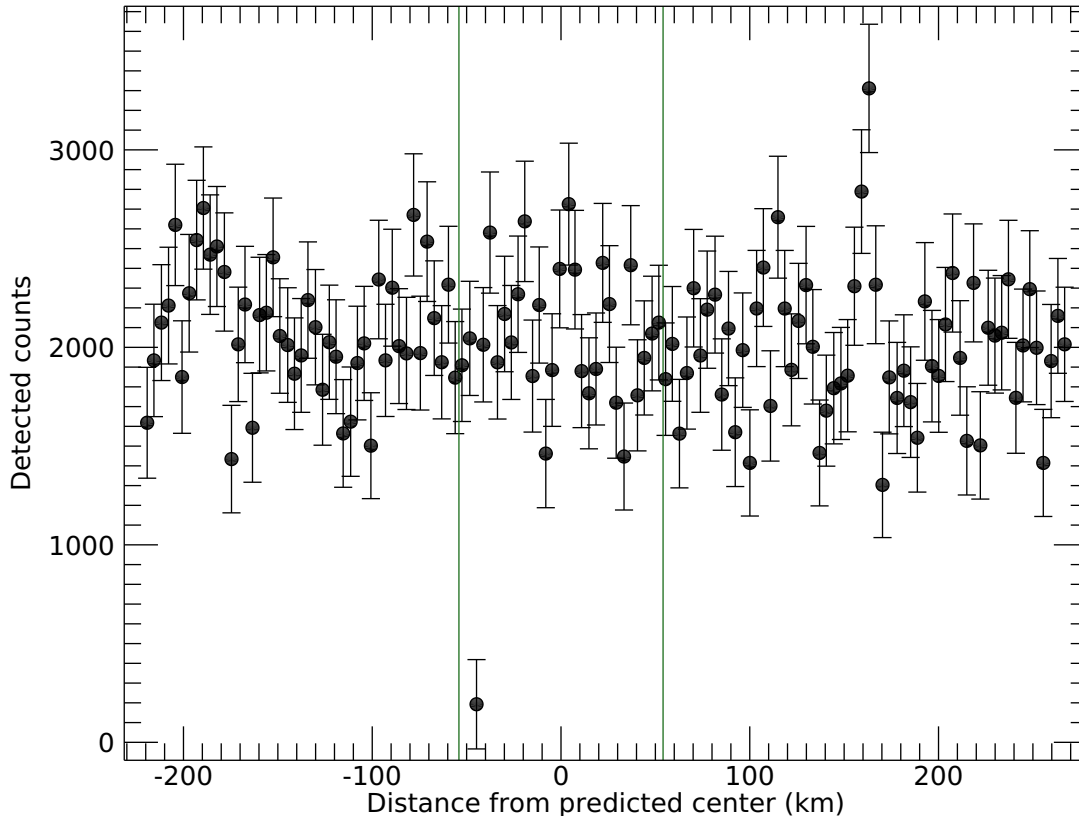
Figure 6. Observations from the 2017-07-10 occultation with SOFIA. The figure shows the lightcurve with a single-point dropout about 45 km prior to the predicted minimum separation. The green vertical lines indicate the predicted 3\text{-}\sigma uncertainty limits for the event. An electronic copy of the data in this figure is provided.
