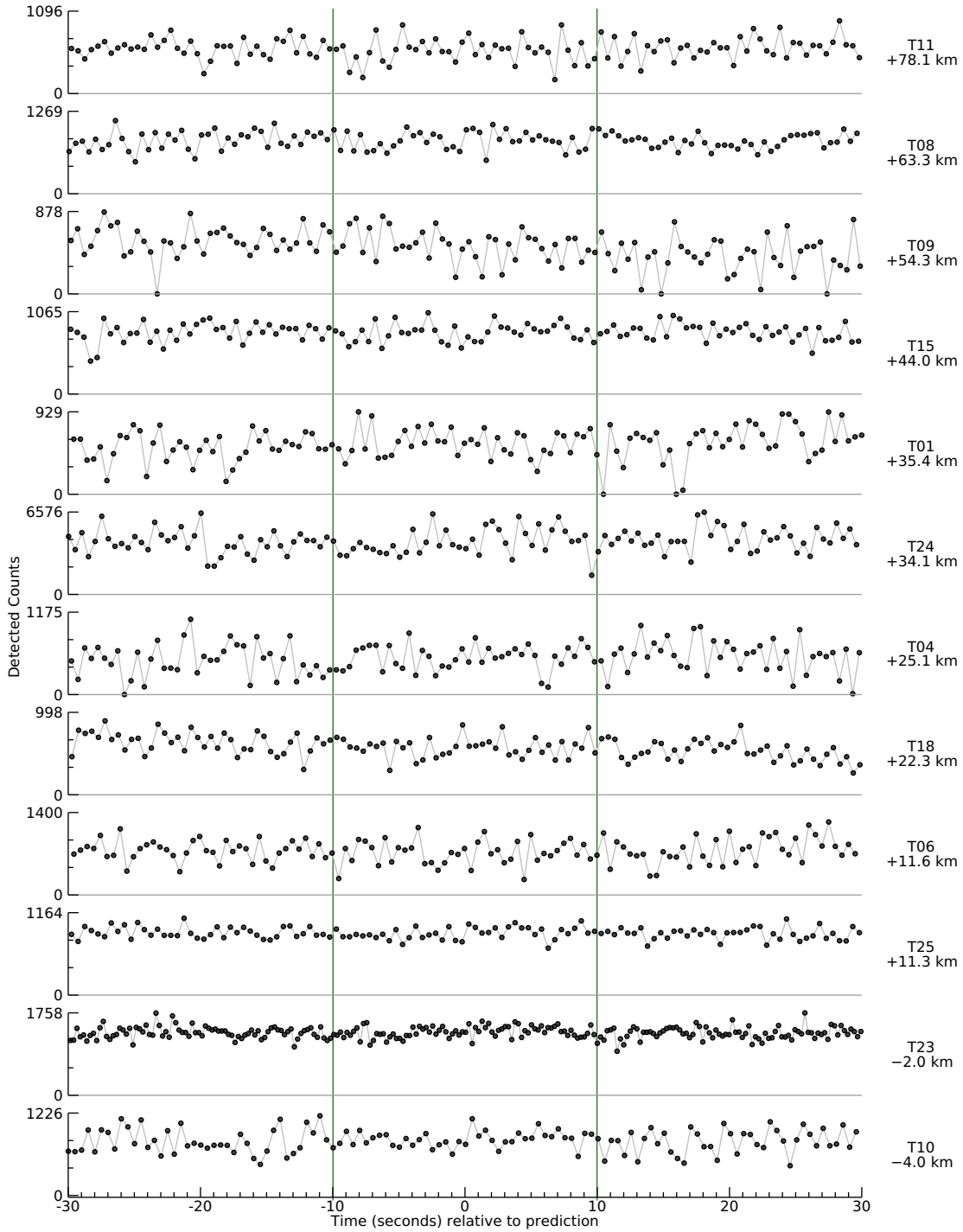
Figure 2. Observations from 2017-06-03 occultation, part 1. The figure shows the lightcurves from the northern half of the data collected by the mobile stations. Each sub-plot is labeled on the right with the team number and the cross-track offset. The team numbers are cross-referenced with Table 2. The plots indicate the signal level from each station – higher numbers indicate higher signal levels. The green vertical lines indicate the predicted 3\text{-}\sigma uncertainty limits for the event. An electronic copy of the data in this figure is provided.
