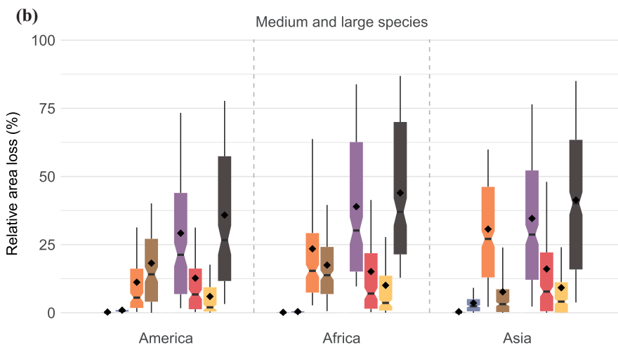
Figure 4. Losses in distribution size for (a) all species and (b) only medium (1–10 kg) and large mammals (>10 kg) due to land use and hunting pressure across the species by continent in 2015 (combined, sum of losses due to land use and hunting minus the overlapping areas; diamonds, mean values per group; lower and upper box boundaries, 25th and 75th percentiles; thick horizontal line, median; notch, 95% CI around estimate of the median; whiskers, 10–90 percentile). Summary statistics are in Supporting Information.
