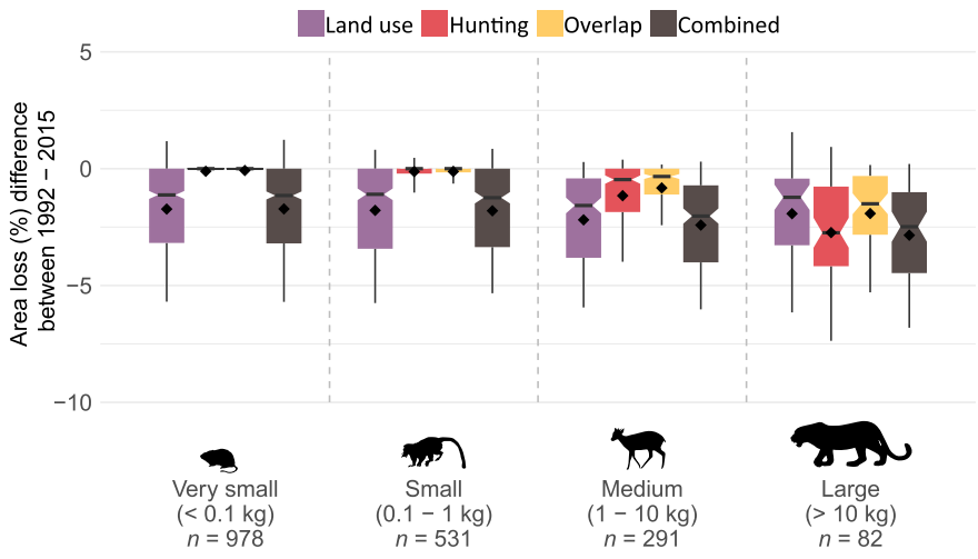
Figure 5. Changes in distribution-size losses due to land use and hunting pressure from 1992 to 2015 (negative values, loss of area from 1992 to 2015; positive values, gain of area; diamonds, mean values per group; lower and upper box boundaries, 25th and 75th percentiles, thick horizontal line, median; notch, 95% CI around the estimate of the median; whiskers, 10–90 percentile). Summary statistics in Supporting Information.
