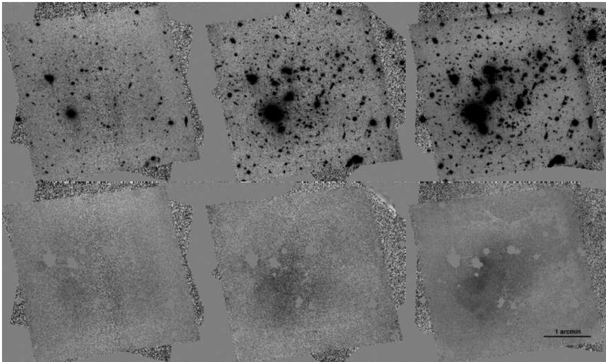
Figure 11. Original images of the relaxed cluster MACS0717 (top) and ICL+background maps provided by CICLE (bottom) in the F435W, F606W, and f814W filters (from left to right). The scale of the original and ICL+background images is the same for each filter.
