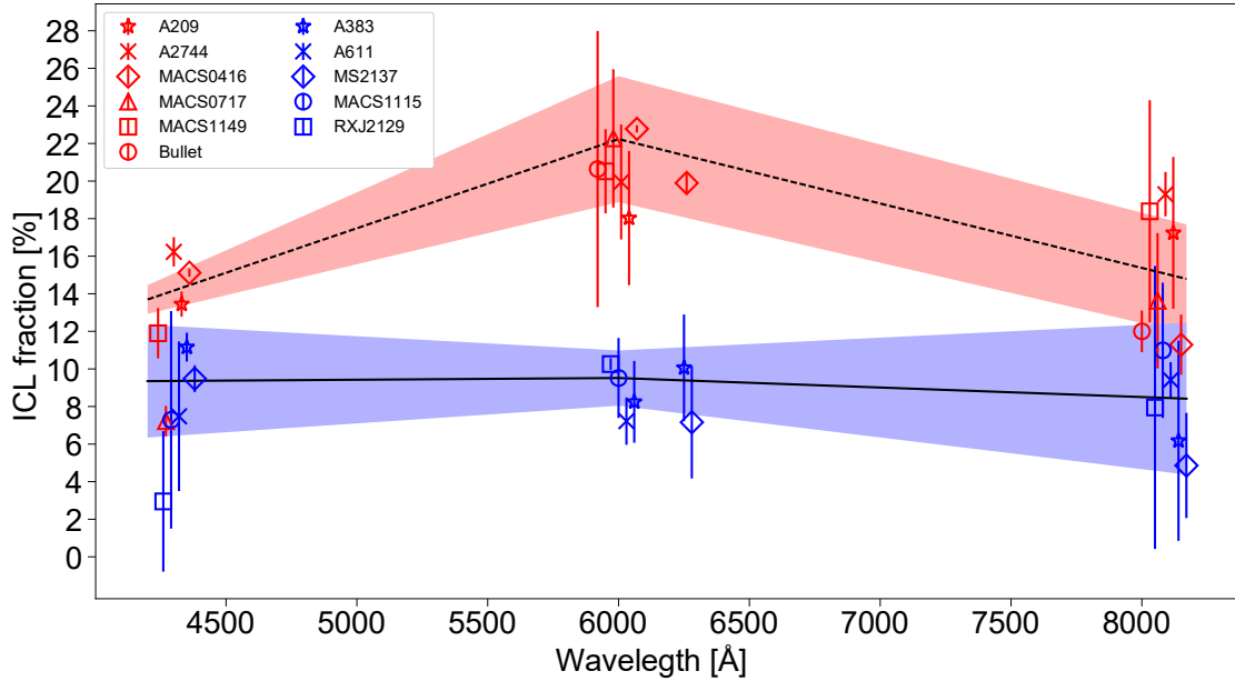
Figure 1. ICL fractions yielded by CICLE for our sample of eleven clusters. Red markers represent merging clusters while blue markers are associated to relaxed systems. The black lines indicate the error weighted mean for each subsample (solid for relaxed clusters and dashed for merging systems), and the shaded areas represent the mean of the errors. For clarity, we have offset horizontally the points by 30 Å gaps.
