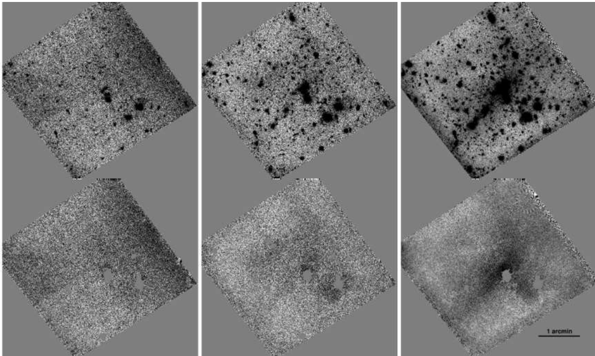
Figure 12. Original images of the relaxed cluster MACS1149 (top) and ICL+background maps provided by CICLE (bottom) in the F435W, F606W, and f814W filters (from left to right). The scale of the original and ICL+background images is the same for each filter.
