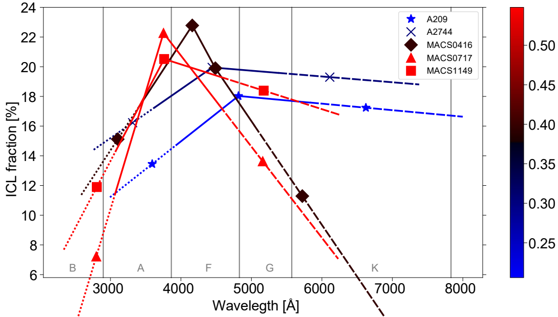
Figure 2. ICL fractions yielded by CICLE for our subsample of merging clusters at rest-frame wavelength. Lines are color coded by redshift and different styles are used to represent the wavelength range covered by each one of the three filters: dotted for the F435W filter, solid for the F606W filter, and dashed for the F814W filter. Vertical gray lines separate the wavelength intervals where the emission peaks of the different stellar spectral types are included, as indicated at the bottom of each region.
