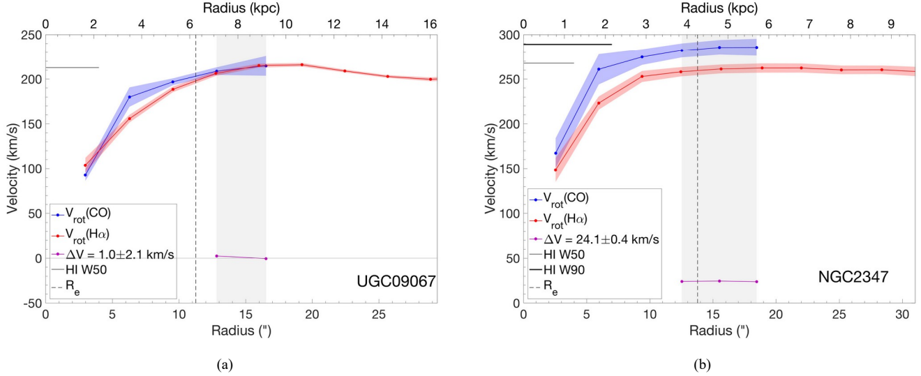
Figure 4. CO and H\alpha rotation curve comparisons for two galaxies. In both plots, V_{\text{rot}}(\text{CO}) is in blue and V_{\text{rot}}(H\alpha) is in red. The purple curves show the difference between the rotation curves at radii greater than R_{\text{beam}} to the furthest CO extent. The median difference between V_{\text{rot}}(\text{CO}) and V_{\text{rot}}(H\alpha) ( \Delta V ) is quoted and the error is the standard deviation. The solid gray and black lines show the inclination corrected V_{\text{rot}}(\text{HI}) values from W50 and W90 for comparison. The black dashed lines show R_e (Table 4). (a) UGC 9067 has CO and H\alpha rotation curves which are consistent within the error bars. (b) NGC 2347 shows a difference of 24 \text{ km s}^{-1} between the CO and H\alpha rotation curves. The HI rotation velocities tend to agree better with the CO rotation curve. Many galaxies in the KSS show \Delta V which are larger than the errors on the rotation curves.
