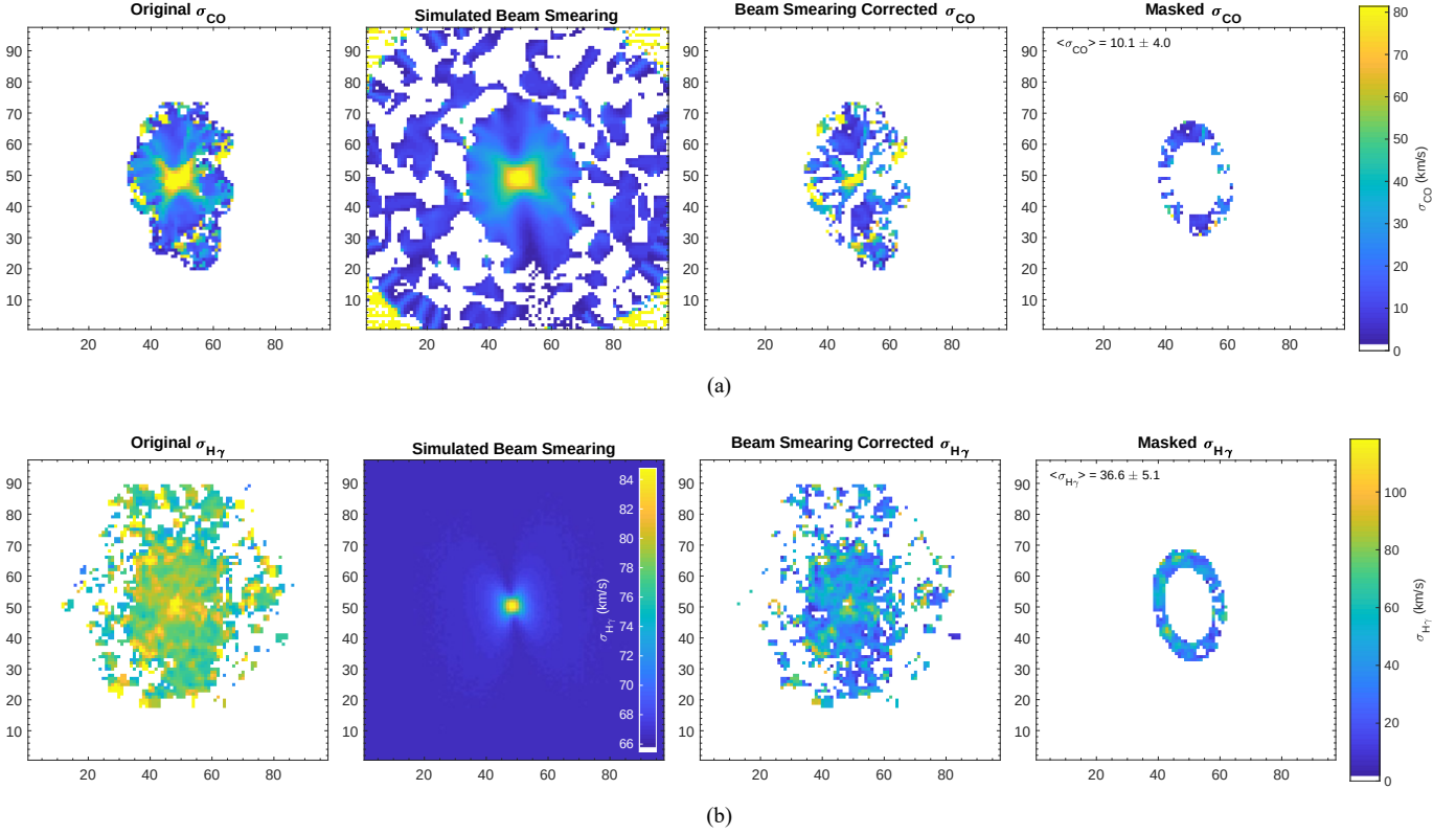
Figure 15. The progression of the beam smearing correction for (a) CO and (b) H V for NGC 2347. From left to right, the panels show the original velocity dispersion map, the simulated velocity dispersion due to beam smearing, the beam smearing corrected velocity dispersion, and the masked beam smearing corrected velocity dispersion. All panels are normalized to the color scales shown to the right, except for the H V simulated beam smearing whose color scale is shown in the inset. White patches in the right two columns are where the simulated beam smearing is larger than the original velocity dispersion and are imaginary when removed in quadrature. These points are discarded for the analysis.
