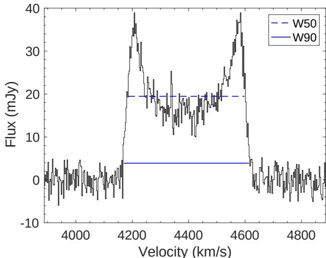
Figure 2. The HI spectrum from the GBT is shown for NGC 2347. The spectrum has been clipped to \pm 500 km s ^{-1} from the CO systemic velocity. The velocities here have been converted to the relativistic convention. Inclination corrected W50 and W90 values are indicated by the dashed and solid blue lines. For this work, the HI data are used as a comparison to the molecular and ionized gas rotation velocities.
