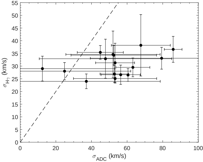
Figure 11. The velocity dispersions inferred from the ADC compared to those measured for the H\gamma emission in each galaxy. The error bars reflect the statistical errors, measured from the standard deviation of the measurements in the annulus. The dashed line is one-to-one. The velocity dispersion \sigma_{H\gamma} is roughly comparable to those inferred from the \sigma_{ADC} ; although \sigma_{H\gamma} tends to be smaller than \sigma_{ADC} this should not be over-interpreted given the difficulty of the measurement discussed in Section 5.5.1.
