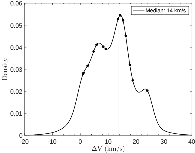
Figure 5. Kernel density estimator showing the distribution of \Delta V (the median V_{\text{rot}}(\text{CO}) - V_{\text{rot}}(H\alpha) ) in the KSS. Each galaxy is represented as a Gaussian with centroid \mu = \Delta V , \sigma = \sigma_{\Delta V} , and unit area. A minimum \sigma_{\Delta V} of 2 \text{ km s}^{-1} is imposed. The Gaussians are summed to produce a histogram and normalized to unit area. The circles indicate the peak of the Gaussian for each galaxy. All galaxies in the KSS have \Delta V > 0 . The median \Delta V is 14 \text{ km s}^{-1} .
