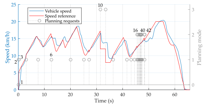
FIGURE 16. Resulting speed profile and planning requests in scenario 2.
