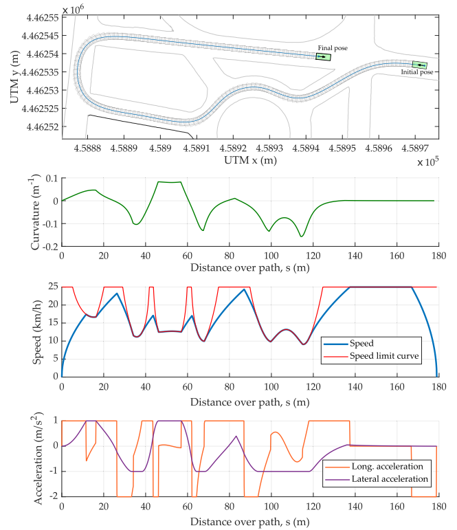
FIGURE 4. In order top-bottom: (i) Example path, (ii) curvature of the path, (iii) speed profile and speed limit curve, and (iv) resulting longitudinal and lateral accelerations.
