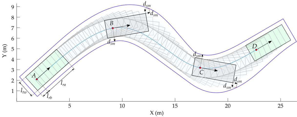
FIGURE 3. Example of the path occupancy polygon calculation for collision checking.
