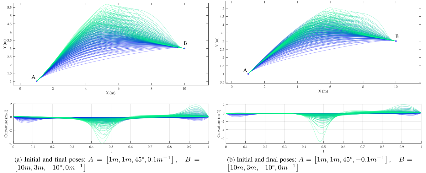
FIGURE 2. Top: Quintic Bézier curves generated with the same initial and final poses. Bottom: Curvatures of the curves.
