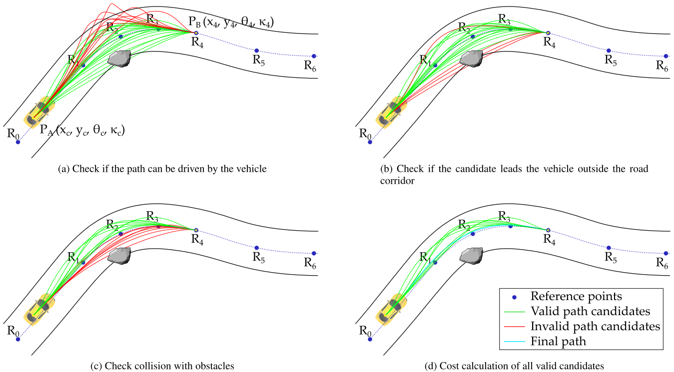
FIGURE 9. Candidates evaluation steps.
