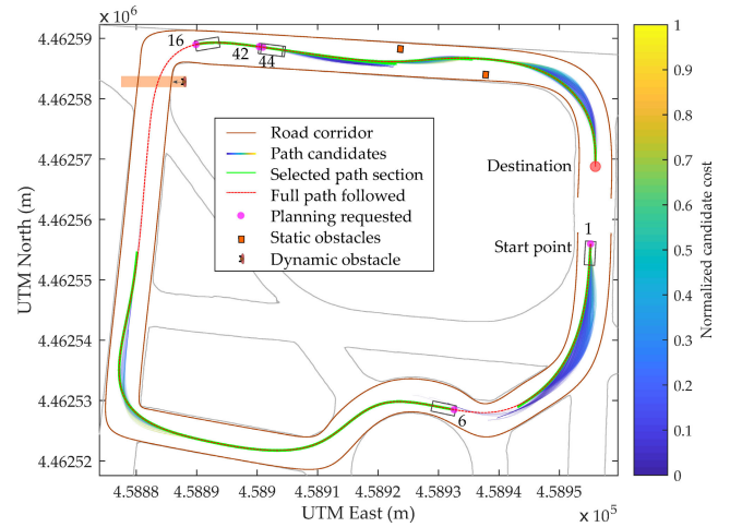
FIGURE 15. Resulting paths in scenario 2.
