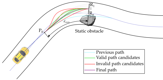
FIGURE 7. Proposed candidates in case a static obstacle must be avoided.
