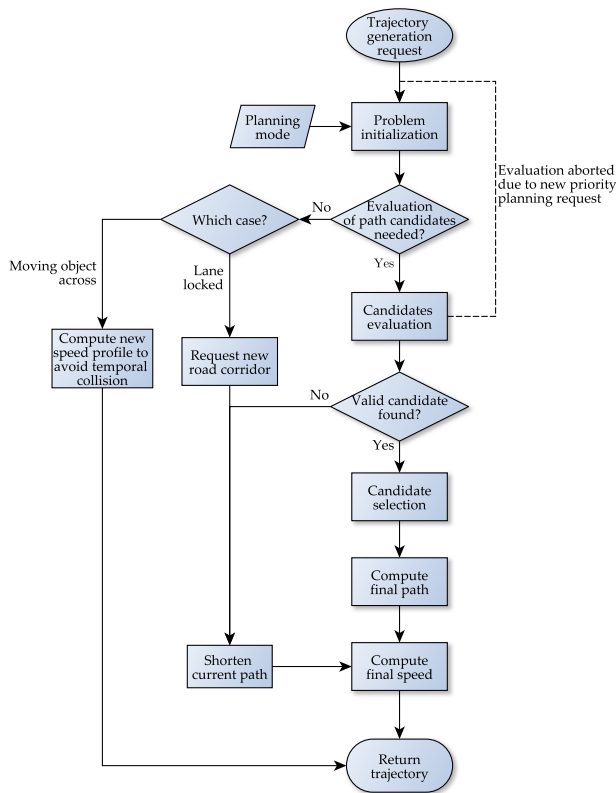
FIGURE 5. General flow diagram of motion planning algorithm.
