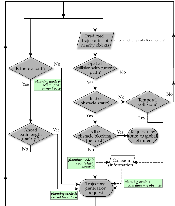
FIGURE 6. Flow diagram of the manoeuvre planner.
