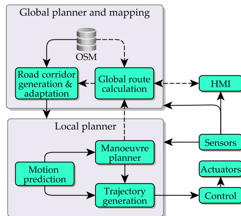
FIGURE 1. Motion planning architecture.
