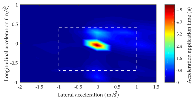
FIGURE 14. Density graph of measured acceleration in the vehicle during the trial in scenario 1.
