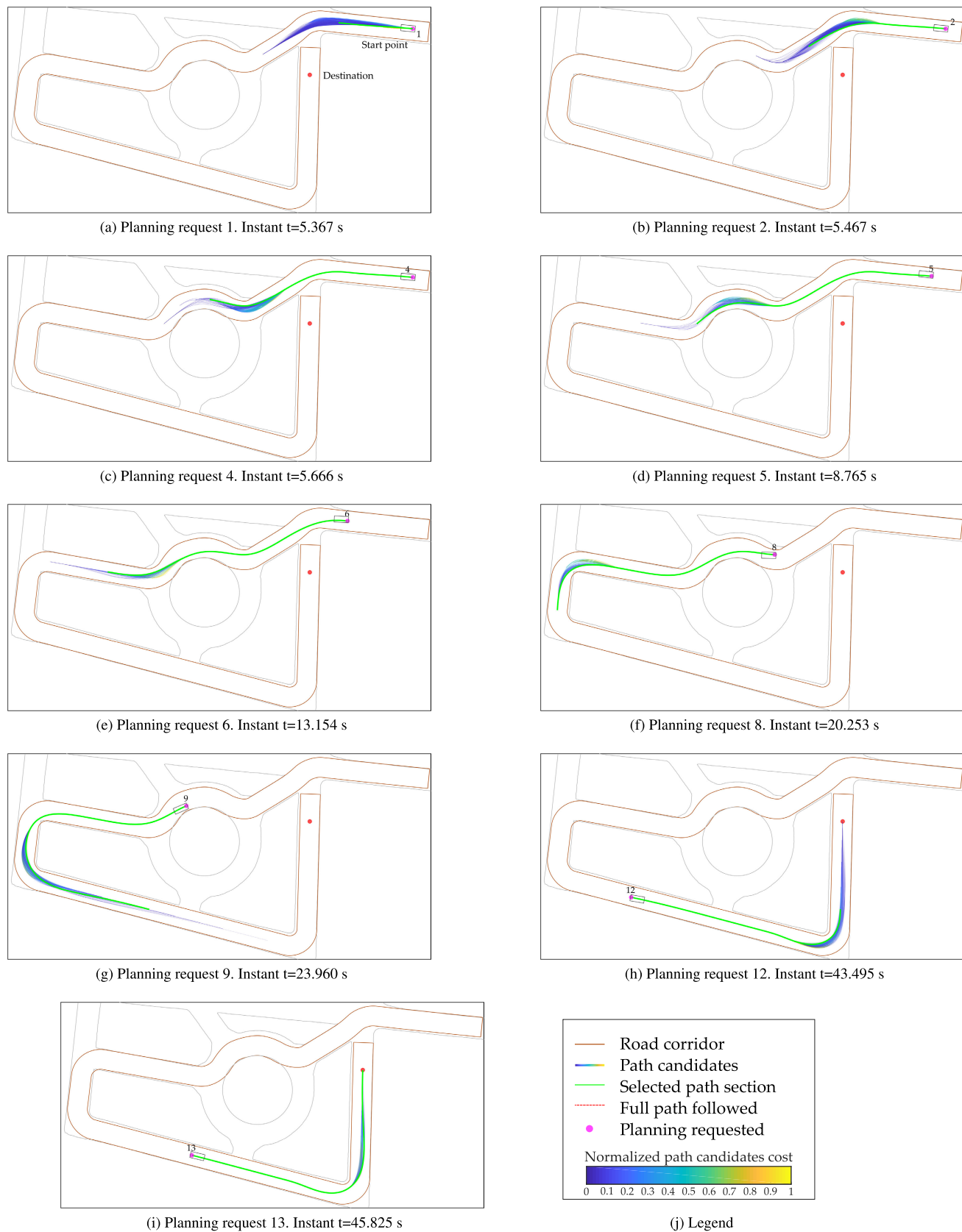
FIGURE 11. Valid and selected candidates at some of the planning requests during the trial in scenario 1.
