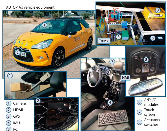
FIGURE 10. Experimental platform.
