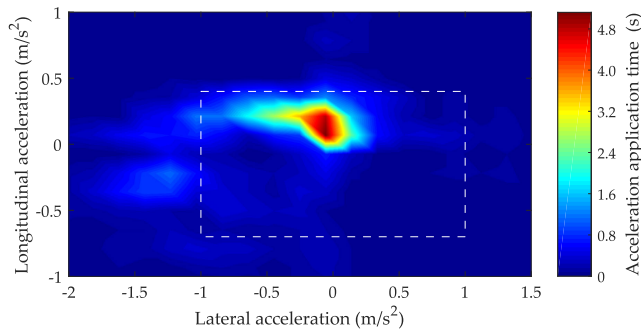
FIGURE 17. Density graph of measured acceleration in the vehicle during the trial in scenario 2.
