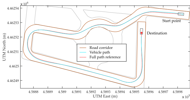
FIGURE 12. Final reference path and vehicle path in the scenario 1.
