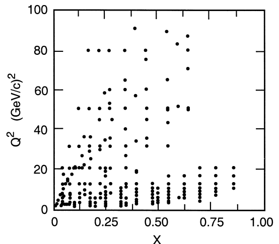
Fig. 2. Kinematic distribution of data used for the R1998 fit.
