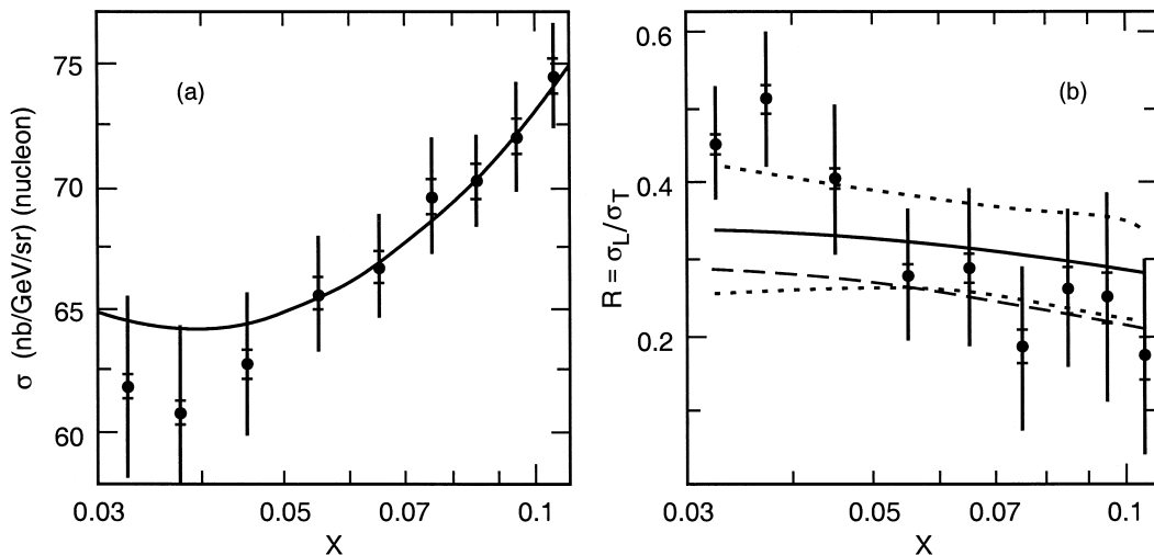
Fig. 1. (a) Cross sections from this experiment (E143) for 29.1 GeV electron scattering from carbon at 4.5^\circ . Inner (outer) error bars are statistical (systematic). The curve is calculated using the NMC fit to F_2 [5], the R1990 fit to R [3], and the A -dependence of lepton-nucleon scattering [6]. (b) R extracted from this experiment (E143) combined with NMC. Inner (outer) error bars are statistical (systematic). The solid curve is the R1990 fit, with the dotted curves showing the error band evaluated at the Q^2 values of the data. The dashed curve is a pQCD calculation described in the text.
