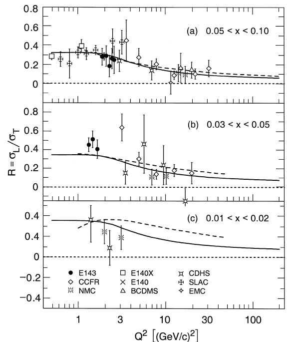
Fig. 3. R as a function of Q^2 for: a) 0.05 \leq x \leq 0.10 ; b) 0.03 \leq x \leq 0.05 ; c) 0.01 \leq x \leq 0.02 . The solid curve is the average of the new fits, R1998, and the dashed curve is the NNLO pQCD calculation described in the text. For clarity, some data points from the same experiment have been combined while others have been shifted slightly in Q^2 .
