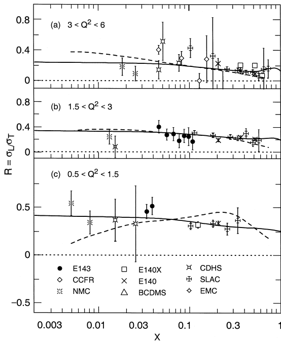
Fig. 4. R as a function of x for: a) 3 \leq Q^2 \leq 6(\text{GeV}/c)^2 ; b) 1.5 \leq Q^2 \leq 3(\text{GeV}/c)^2 ; c) 0.5 \leq Q^2 \leq 1.5(\text{GeV}/c)^2 . The solid curve is the average of the new fits, R1998 , and the dashed curve is the NNLO pQCD calculation described in the text. For clarity, some data points from the same experiment have been combined while others have been shifted slightly in x .
