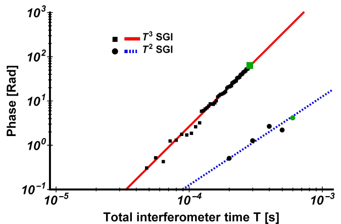
FIG. 3. Comparison between the scalings of the interferometer phases \delta\Phi^{(T^3)} (solid red curve) and \delta\Phi^{(T^2)} (dashed blue curve) given by Eqs. (10) and (11), respectively. The squares are data from Fig. 2, while the dots are from our T^2 -SGI realization [11]. The green square represents the largest accumulated phase of the T^3 -SGI in its current configuration with T_{\max} = 285 \mu\text{s} at the point of \approx 30\% contrast. As a reference, the green dot indicates the largest accumulated phase observed with a T^2 -SGI also at \approx 30\% contrast. The latter is significantly smaller although the magnetic field gradients and the maximal time T_{\max} = 924 \mu\text{s} are larger than those of the T^3 -SGI by a factor of 2.3 and 3.2, respectively [36].
