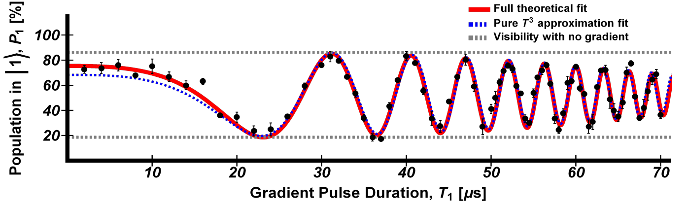
FIG. 2. Measurement of the cubic phase with the T^3 -SGI presented in Fig. 1. The solid red line represents a fit based on Eqs. (8) and (9) to the experimental data (dots), where the fitting parameters are the decay constant, the magnetic acceleration a_B , and a constant phase \varphi_0 . The dashed blue line is a fit based on Eq. (9) with T_d = 0 , leading to a pure T_1^3 scaling of the interferometer phase as seen in Eq. (10). The visibility drops from 68% to 32% over 70 \mu\text{s} with a decay time of 75 \mu\text{s} . This reduction results from inaccuracies in recombining the two interferometer paths. The dashed gray horizontal lines depict the maximal and minimal values of the population P_1 measured without magnetic field gradients.
