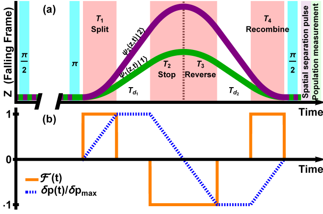
FIG. 1. Pulse sequence of our longitudinal T^3 -SGI (not to scale). (a) Center-of-mass trajectories of the atomic wave packets with internal states |1\rangle (bottom, green) and |2\rangle (top, purple). Also shown are the \pi/2 and \pi RF (light blue) and magnetic gradient splitting, stopping, reversing and recombining pulses (light red). The magnetic field gradients result in a state-dependent force along the z -direction while the strong bias magnetic field along the y -direction defines the quantization axis. (b) Time-dependence of the relative force \mathcal{F} \equiv \mathcal{F}(t) , Eq. (3), (orange curve) and the corresponding relative momentum \delta p(t) = \mathcal{P}_2(t) - \mathcal{P}_1(t) , (blue dashed curve) between the wave packets moving along the two interferometer paths. In the experiment, we have achieved the maximal separations \delta z_{\max} = 1.4 \mu\text{m} and \delta p_{\max}/m_{Rb} = 19 \text{ mm/s} in position and velocity.
