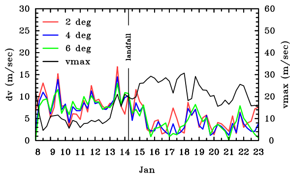
Figure 5. Mean vertical wind shear, characterized by the magnitude of the vector velocity difference between 850 mb and 200 mb, averaged over boxes 2^\circ\text{lon} \times 2^\circ\text{lat} , 4^\circ\text{lon} \times 4^\circ\text{lat} , and 6^\circ\text{lon} \times 6^\circ\text{lat} centred on the location of the minimum geopotential at 850 mb and maximum wind speed at 850 mb within the 2^\circ\text{lon} \times 2^\circ\text{lat} box.
