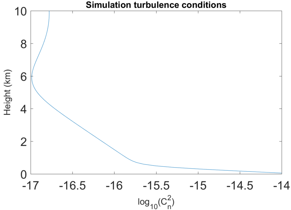
FIGURE 6.1 The typical vertical C_n^2 profile of Monterey, CA, created by LEEDR. This profile is used for the laser simulations in this chapter.
