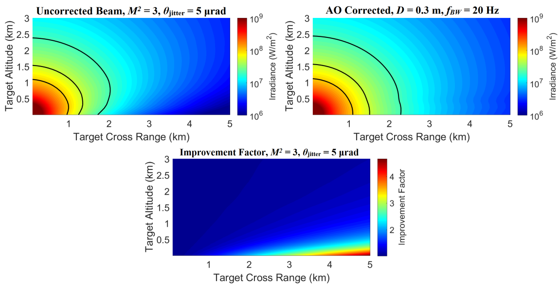
FIGURE 6.8 Peak irradiance plots for uncorrected and AO compensated laser beams where f_{BW} = 20 \text{ Hz} and D = 0.3 \text{ m} . The laser beam source is described by M^2 = 3 and has 5 \mu\text{rad} of uncorrected platform jitter. The maximum improvement factor is approximately 5.
