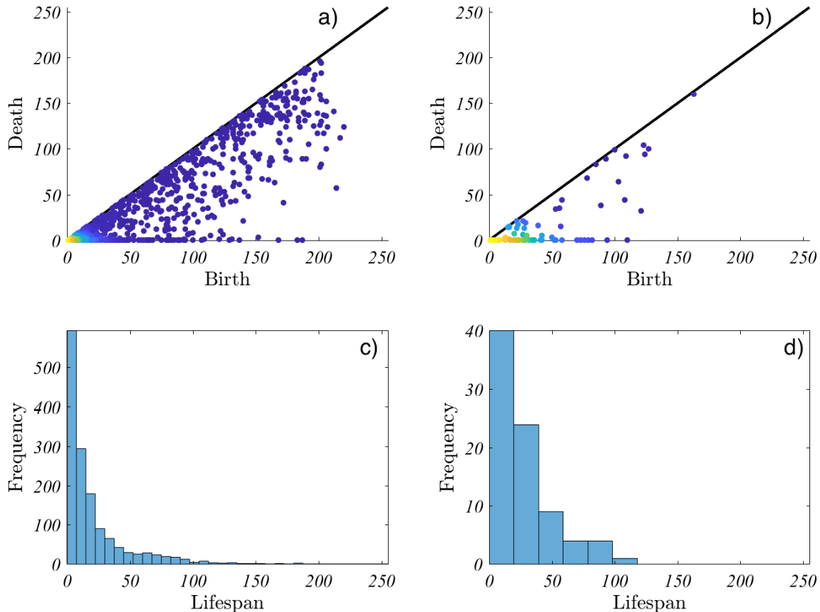
FIG. 2. Persistence diagrams (PDs) for the reference experiment (medium 6.25 – 4.5) (same time as shown in Fig. 1). The parts (a) and (b) show the PDs for components and loops, PD_0 , and PD_1 , respectively. The parts (c) and (d) show the corresponding lifespans. The x -axis range correspond to brightness, covering the full range [0 : 255] . Note large number of generators with very small lifespans, showing that there are many points in the diagrams that are near the diagonals and represent essentially noise. Supplementary animation [45] show the PDs and lifespans for all considered images of the reference experiment.
