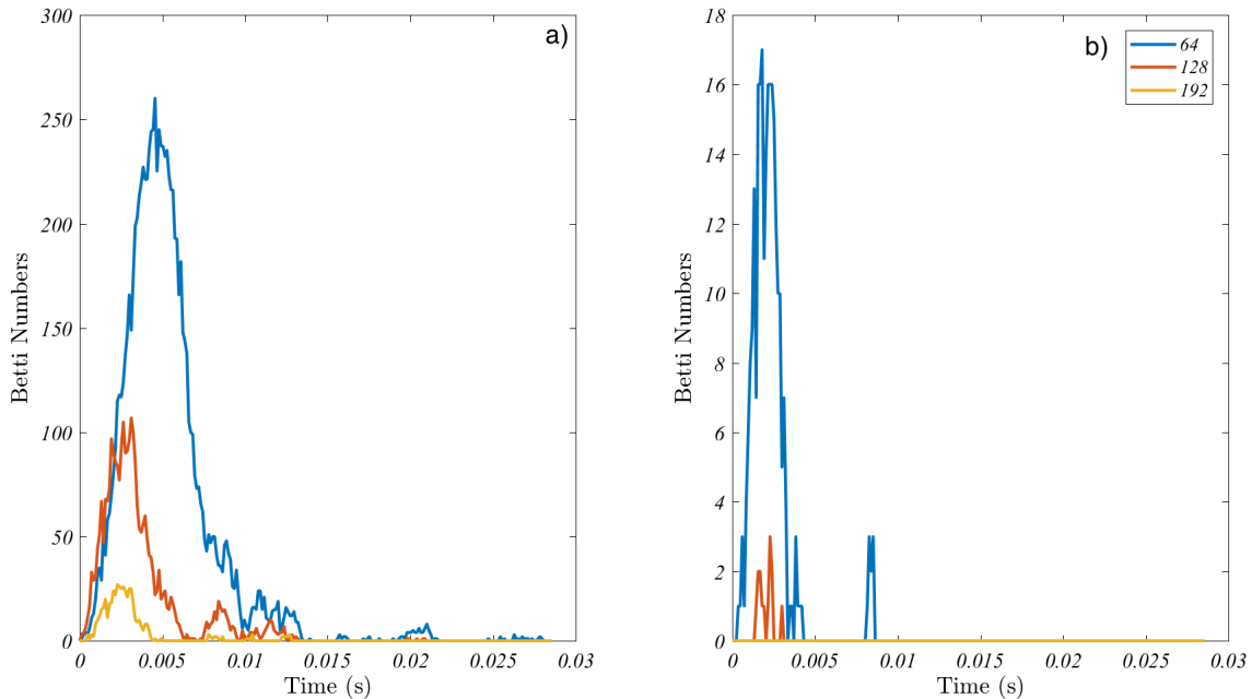
FIG. 4. Betti numbers, \beta_0 (a) and \beta_1 (b), for the reference case, respectively. No smoothing is used here since the amount of data particularly for \beta_1 , is limited. The results are shown for three different brightness threshold levels, as discussed in the text.
