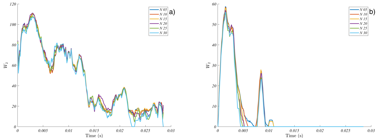
FIG. 6. Wasserstein distance between the consecutive images for the reference case as a different amount of noise (shown by the values of N in the legends) is assumed for components (a) and loops (b). The distances are essentially insensitive to noise.
