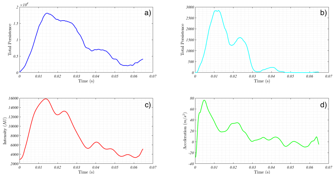
FIG. 5. Total persistence, for the components, TP_0 , for the loops, TP_1 , photoelastic response, and intruder's acceleration for the impact on soft particles (soft 6.35 – 1.3).
