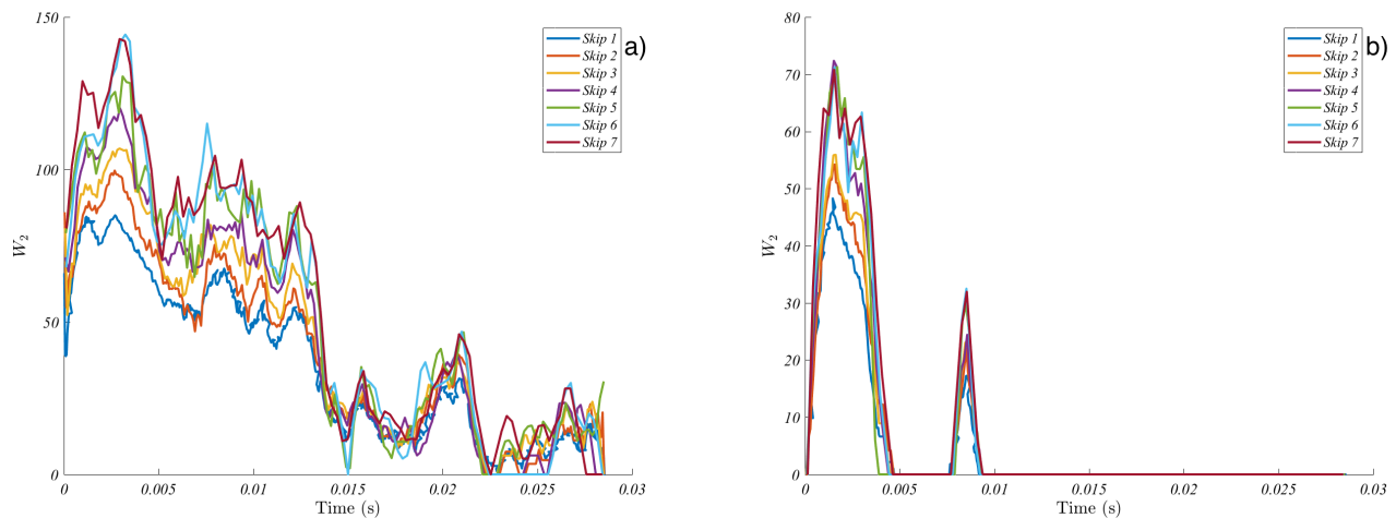
FIG. 7. Wasserstein distance between the images for the reference case assuming that the generators closer than 30 pixels to the diagonal can be ignored. The given number of ‘skips’ specifies the number of images that were skipped in the calculation of the Wasserstein distance. The part (a) shows the results for components, and the part (b) for loops.
