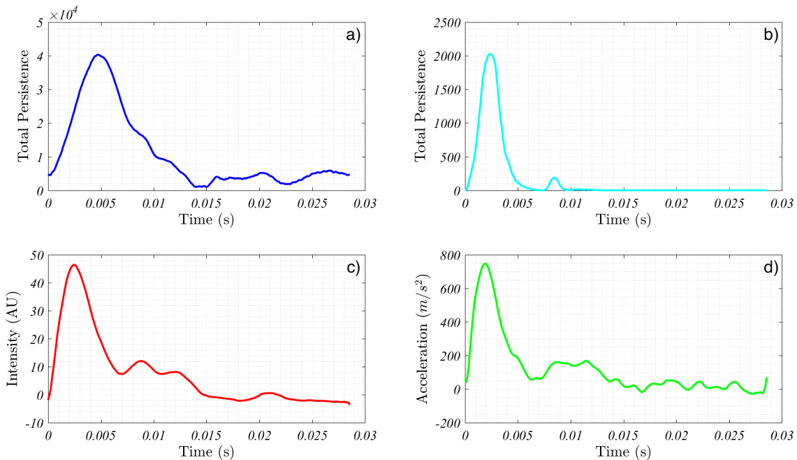
FIG. 3. Total persistence, for the components, TP_0 , for the loops, TP_1 , photoelastic response, and intruder’s acceleration for the reference case (medium 6.35 – 4.9). Supplementary animation [46] shows the above curves jointly with the (processed) photoelastic images.
