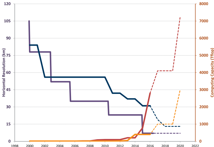
FIG. 2. Historical (solid) and projected (dashed) computing capacity (teraflops) and global model resolution (km) for NOAA (red/purple) and the U.S. Navy (gold/blue). Data courtesy of NCEP Office of Central Processing ( www.emc.ncep.noaa.gov/gmb/STATS/html/model_changes.html ) and the NRL/MRY.
