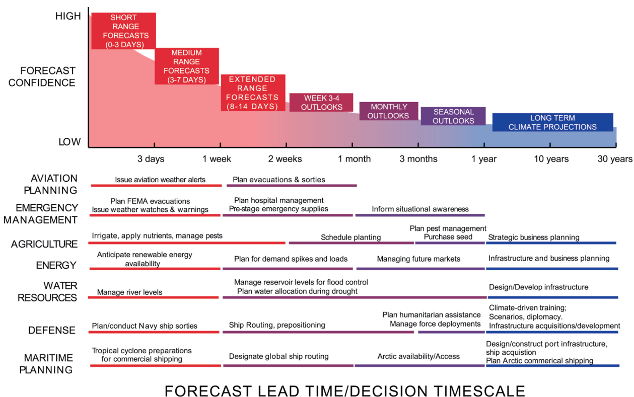
FIG. 1. Sampling of federal decision needs across time scales. Decisions span weather to climate prediction/projection capabilities, with responsibilities for actions falling throughout the federal and commercial sectors. Adapted from NRC (2016).
