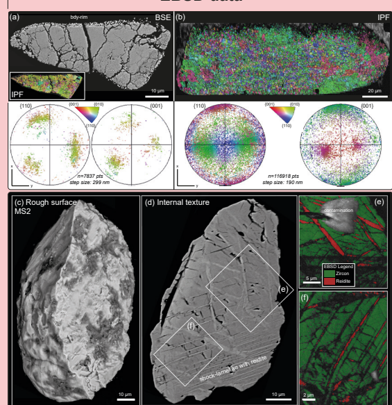
Figure 3. EBSD analyses: granular zircons with baddeleyite rim(?) from (a) melt-bearing impact breccia (thin section) and (a) impact-melt (separate), yields three main clusters with high angle arrangements towards each other – coinciding between {001} and {110} pole projections (fig. 3a and 3b; IPF colours represent neoblast orientations), indicative of FRIGN zircon. BSE-images on rough surface (c) and internal texture (d) of zircon MS2 from the melt-bearing impact breccia (3). EBSD analysis indexing reidite within several intersecting planar shock-lamellas (fig. 3e-f).
