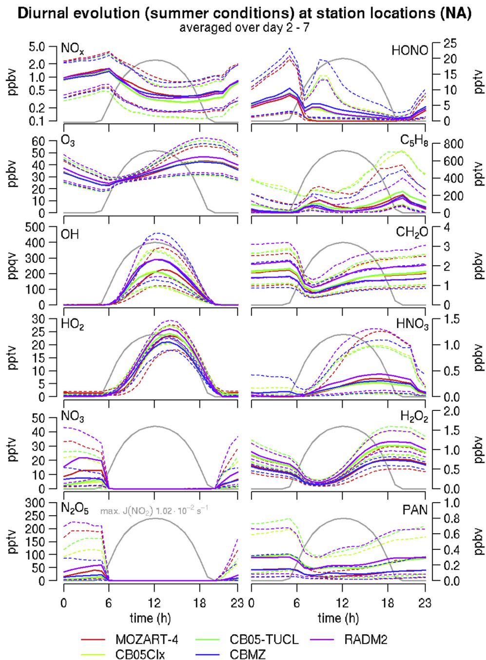
Fig. 5. 25 (dashed), 50 (solid) and 75 (dashed)% values for select species as result of the box model runs under 'summer' conditions at the observation locations used in Im et al. (2015) for the North American domain. Different colors represent different mechanisms. Gray line is J(\text{NO}_2) (units not shown). Note logarithmic scale for \text{NO}_x . PAN is sum of all PAN species (MOZART-4: PAN + MPAN, CB05Clx: PAN + PANX, CB05-TUCL: PAN + PANX + OPAN, CBMZ: PAN, RADM2: PAN + TPAN).
