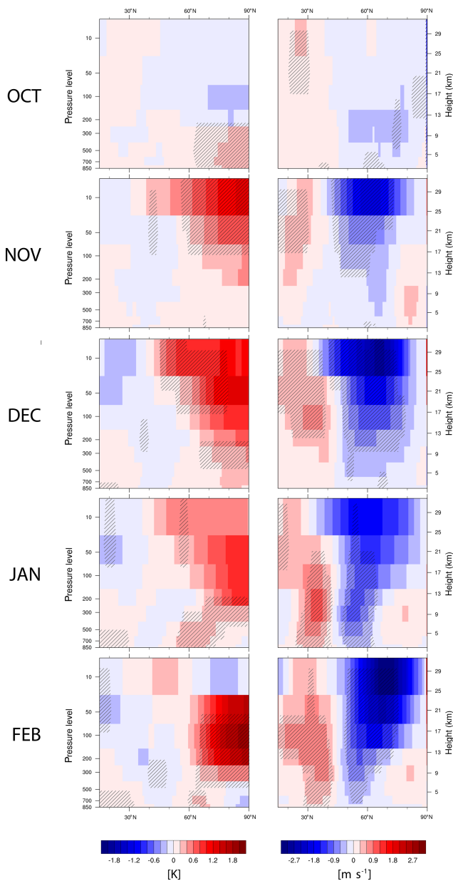
Figure 4. Zonal mean ( 180^{\circ}\text{E} – 180^{\circ}\text{W} , 15 – 90^{\circ}\text{N} ) (left) temperature anomalies and (right) zonal mean zonal wind anomalies projected onto snow indices in November for ERA20C covering 1901–2010. Shading indicates 95 % significance level.
