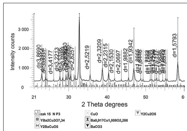
Figure 3 XRD analysis of the TP-3 sample
