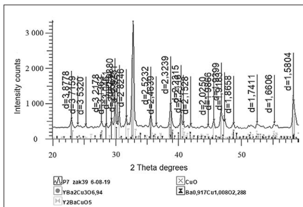
Figure 1 XRD analysis of MP-1
