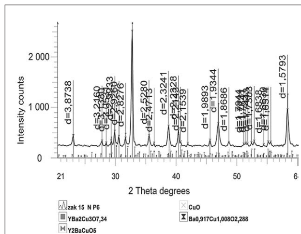
Figure 4 XRD analysis of the TP-6 sample
