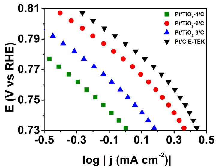
1 2 Figure 4. Tafel plots for Pt/TiO 2 -1/C (green trace), Pt/TiO 2 -2/C (red trace), Pt/TiO 2 -3/C (blue 3 trace) and Pt/C E-TEK (black trace). The data was normalized by the geometric area of the 4 electrode and calculated from their corresponding rotating disk electrode values at 1600 rpm. 5
