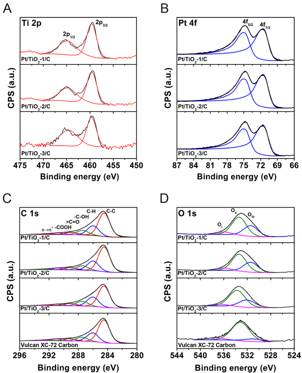
1 2 Figure 2. Deconvoluted X-ray photoelectron spectra (XPS) of the Ti 2p (A), Pt 4f (B), C 1s (C), 3 and O 1s (D) core levels for Pt/TiO 2 -1/C, Pt/TiO 2 -2/C, Pt/TiO 2 -3/C, Vulcan XC-72 carbon (top to 4 bottom traces, respectively).
