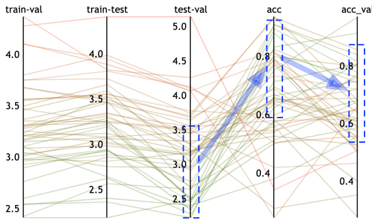
Figure 8: The influence of topological distance among training, validation, and test set on the prediction accuracy. The first three axes represent \bar{d}_{(train, val)} , \bar{d}_{(train, test)} , and \bar{d}_{(test, val)} of each student. The last two axes denote the average personal accuracy of each student on their test and validation set, respectively. Each line represents the data of one student and the line color indicates the value of \bar{d}_{(test, val)} (the green to red scheme denotes the small to large values).
