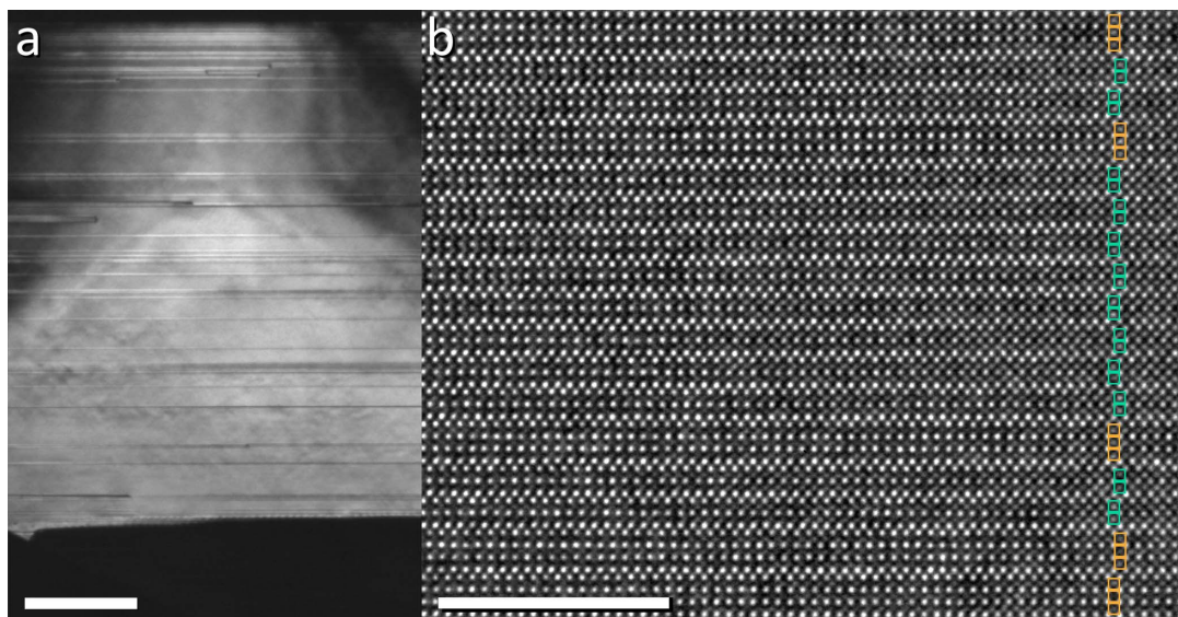
Fig. 2. Transmission electron micrographs of \text{Ca}_3\text{Mn}_2\text{O}_7 at the [110] A2_1am zone axis. a) Dark field 220 image showing planar defects and contrast bands in a single grain (scale bar 200 nm). b) High resolution [110] lattice image showing the occurrence of n = 3 perovskite blocks forming planar defects. Scale bar 10 nm.
