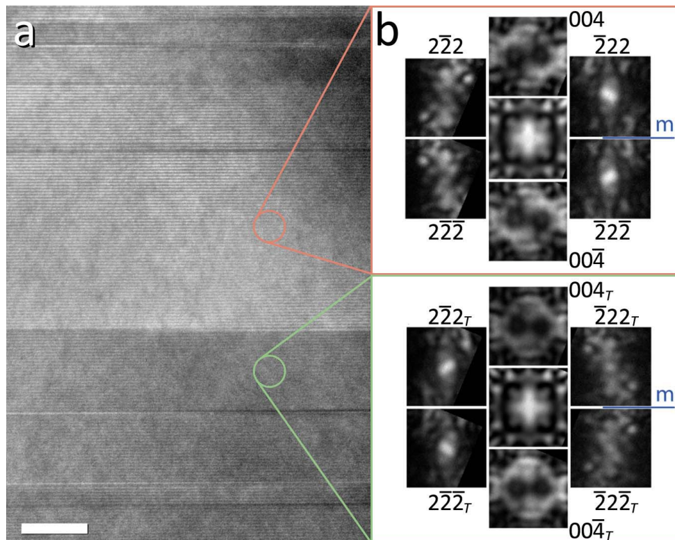
Fig. 5. a) contrast bands in a TEM image of \text{Ca}_3\text{Mn}_2\text{O}_7 close to the [1\bar{1}0] axis. b) Selected D-LACBED patterns taken from different bands showing that the structures are related by a twinning operation such as a (110) mirror or an inversion, although it is not possible to distinguish between them.
