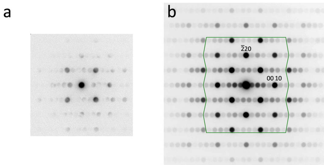
Fig. 3. a) Individual RT CBED pattern obtained at the \text{Ca}_3\text{Mn}_2\text{O}_7 [1\bar{1}0] A2_1am zone axis. b) Average RT CBED pattern, the sum of 3,721 CBED patterns. The 109 spots used to reconstruct D-LACBED patterns lie inside the green boundary.
