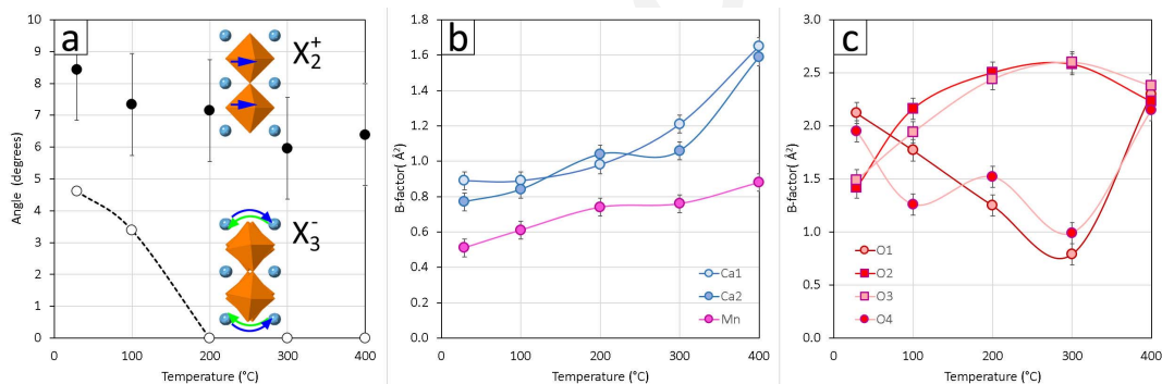
Fig. 9. (a) The magnitude of oxygen octahedral rotations corresponding to the distortion modes X_3^- and X_2^+ (or X_1^- ). (b) Thermal atomic displacement parameters ( B -factors) for Ca and Mn as a function of temperature. (c) B -factors for oxygen atoms showing an anomalous decrease for O1 and O4 up to 300°C.
