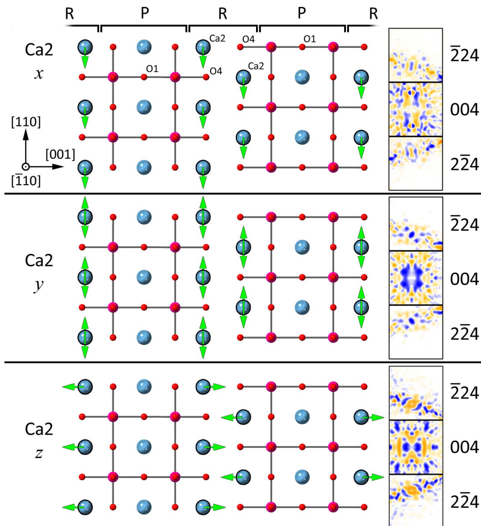
Fig. 7. Left: the movements of atom Ca 2 from the prototype structure within space group A2_1am when displaced along the x , y and z direction respectively as seen in the [1\bar{1}0] projection. Colour coding is Ca blue, Mn magenta and oxygen red; perovskite/rocksalt layers are labelled P and R respectively. There are eight symmetrically equivalent Ca 2 atoms in the unit cell, which lie in the rocksalt layers, while Ca 1 atoms lie in the perovskite layers. Right: three \delta_{ij} patterns ( \bar{2}24 , 004 , 2\bar{2}4 ) showing the resulting changes in intensity (yellow = positive, blue = negative). Displacement of Ca 2 along x breaks mirror symmetry and produces antisymmetric \delta_{ij} patterns. Displacement of Ca 2 along y moves atoms at different depths in opposite directions, maintaining mirror symmetry in the projection and \delta_{ij} patterns, while displacement along z moves Ca 2 away from the perovskite layers, also maintaining mirror symmetry. See also video V1 and figure ?? in the appendix.
