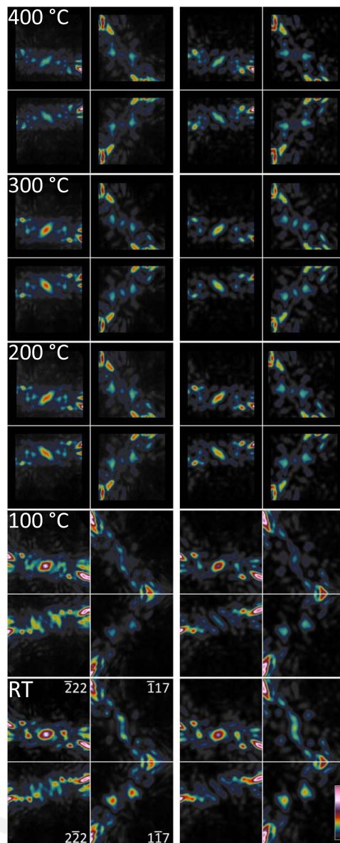
Fig. 8. Comparison of experimental D-LACBED patterns (left) and best-fit simulated LACBED patterns (right) at a range of temperatures. The \bar{2}22 and \bar{1}17 Bijvoet pairs are strongly asymmetric at RT due to the presence of both X_2^+ and X_3^- distortions (see Fig. 1). Mirror symmetry is present at 200°C and higher.
