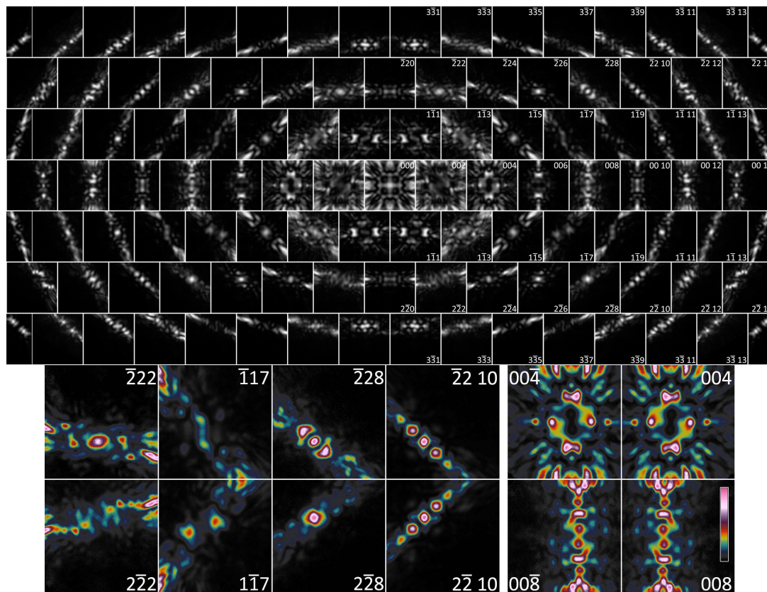
Fig. 4. Top: the 109 experimental RT (29°C) D-LACBED patterns at the \text{Ca}_3\text{Mn}_2\text{O}_7 [\bar{1}\bar{1}0] zone axis corresponding to the spots indicated in Fig. 3b. All patterns have an angular range of 20 mrad and are normalised to the full intensity range for display. A mirror is present on (001) but not (110), which can be seen in 00h patterns and by comparing Bijvoet pairs \bar{h}hl and h\bar{h}l (false colour patterns, bottom).
