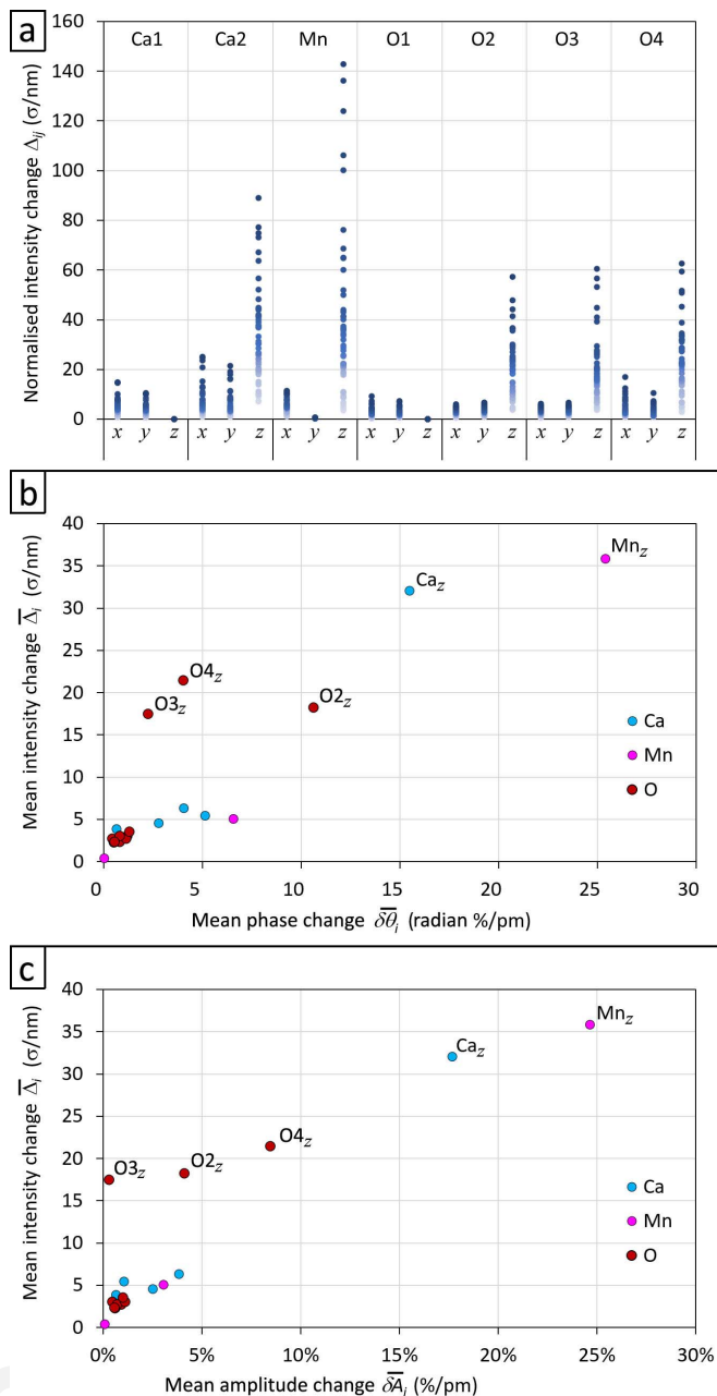
Fig. 6. a) Normalised RMS changes in intensity \Delta_{ij} of the 54 unique [110] LACBED patterns for the 19 allowed atom displacements within the constraints of A2_1am (N.B. Ca1 z and O1 z are fixed at zero). The change in intensity is given in units of standard deviation of the image per nm movement. b) The correlation between the average of all LACBED intensity changes \bar{\Delta}_i and the average change in structure factor phase \bar{\delta}\theta_i for the 19 allowed atom displacements. c) The same correlation for the mean change in structure factor amplitude \bar{\delta}A_i .
