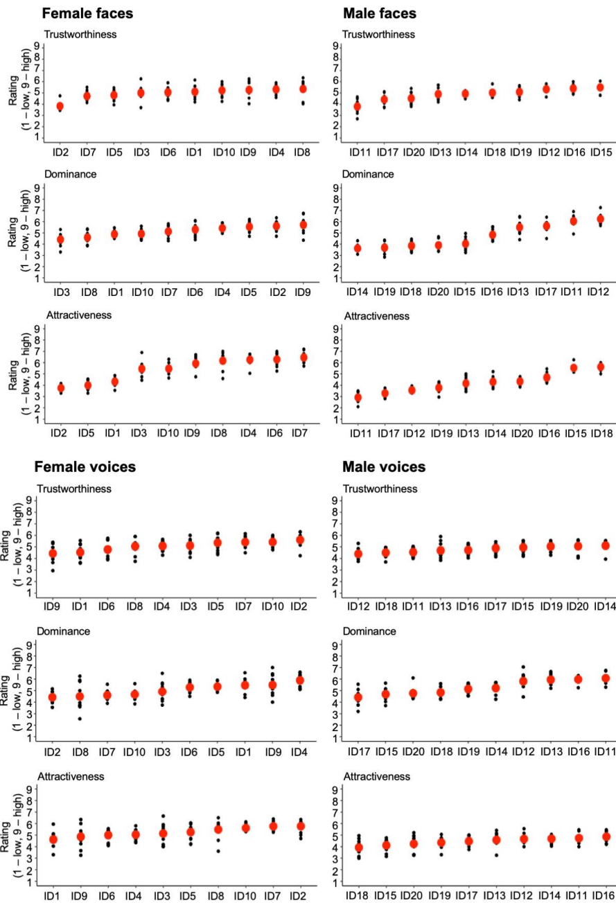
Supplementary Figure 4: Mean trait ratings plotted per item (black dots) and per identity (red dots). Higher within-person variability is indicated by a larger range in mean ratings per item. Higher between-person variability by a larger range of mean ratings per identity.
