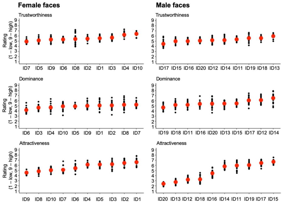
Supplementary Figure 1: Mean trait ratings plotted per item (black dots) and per identity (red dots). Higher within-person variability is indicated by a larger range in mean ratings per item. Higher between-person variability by a larger range of mean ratings per identity
