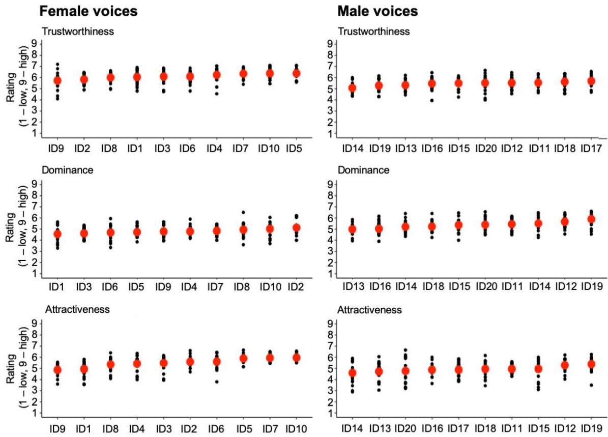
Supplementary Figure 2: Mean trait ratings plotted per item (black dots) and per identity (red dots). Higher within-person variability is indicated by a larger range in mean ratings per item. Higher between-person variability by a larger range of mean ratings per identity
