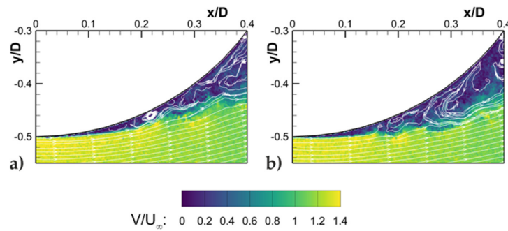
Figure 10. Instantaneous velocity magnitude and streamlines at Re = 1.69 \times 10^5 , showing the intermittency of the separation bubble (equivalent bowling speed of 78 mph).
