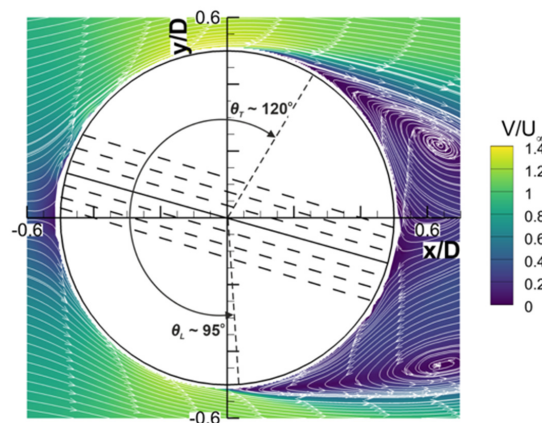
Figure 8. Time-averaged velocity magnitude and streamlines at U_\infty = 12 m/s, Re = 1.1 \times 10^5 (equivalent bowling speed of 54 mph), showing conventional swing, on the seam side \theta_T \sim 120^\circ and on the non-seam side \theta_L \sim 95^\circ . Separation angles shown to nearest 5^\circ .
