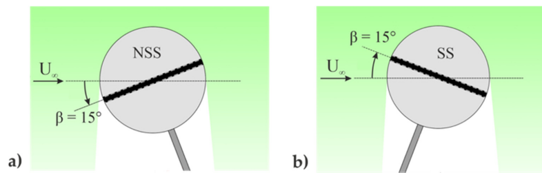
Figure 7. Position of the ball to investigate (a) the non-seam side (NSS) and (b) the seam side (SS).
