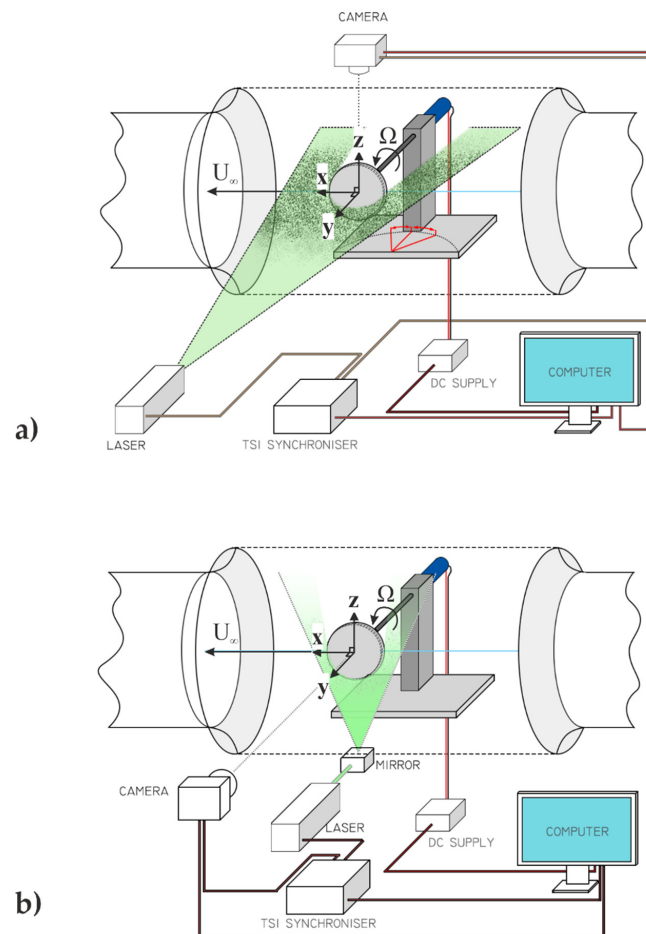
Figure 6. Experimental configuration of (a) the horizontal plane to investigate swing, and (b) the vertical plane to investigate the Magnus effect. Flow is from right to left.
