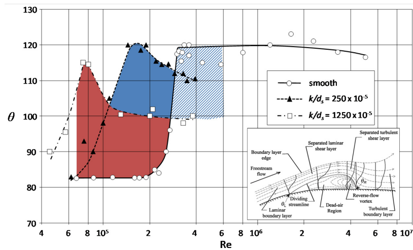
Figure 2. Variation of separation angles (with respect to the stagnation point) for smoothed and roughened spheres. Red represents the difference in separation angle either side of the ball during conventional swing (CS); solid blue shows reverse swing (RS) on an old ball and hatched blue denotes RS on a new ball. Triangles represent roughened non-seam side (NSS) and squares represent seam roughness.
