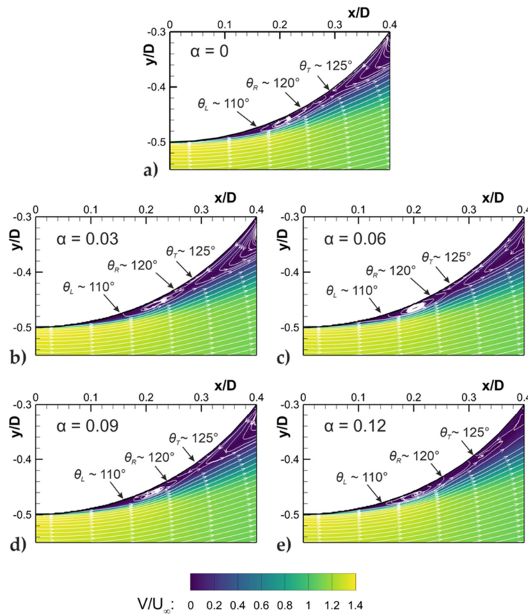
Figure 11. Time-averaged velocity magnitude and streamlines at Re = 1.69 \times 10^5 on the NSS for different spin rates, \alpha (equivalent bowling speed of 78 mph). Separation and reattachment angles shown to nearest 5^\circ .
