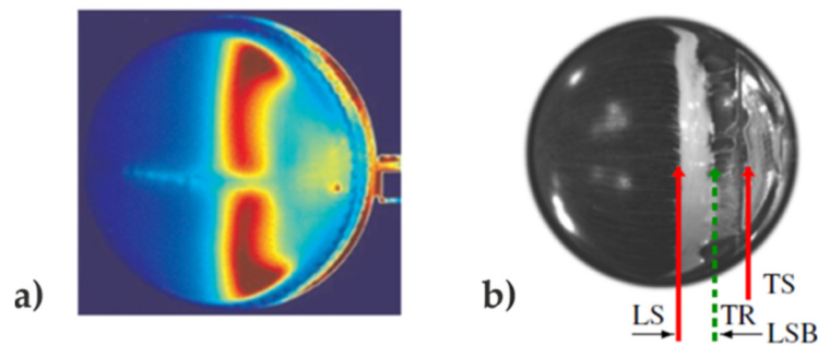
Figure 4. Evidence of a laminar separation bubble on the NSS using two different methods: (a) heat flow method on a double-sized cricket ball model [5] and (b) oil flow visualization on a sphere with a trip [14].
