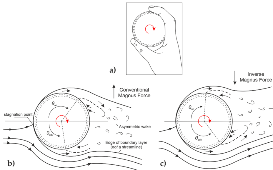
Figure 5. (a) Side-on illustration of a bowler's grip on a cricket ball showing direction of spin; (b) conventional Magnus force; and (c) inverse Magnus force.
