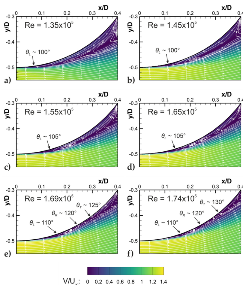
Figure 9. Time-averaged velocity magnitude and streamlines with varying Re at a magnified region on the non-seam side, showing the formation of the separation bubble at \alpha = 0 (equivalent bowling speeds between 62 and 81 mph). Separation and reattachment angles shown to nearest 5°.
