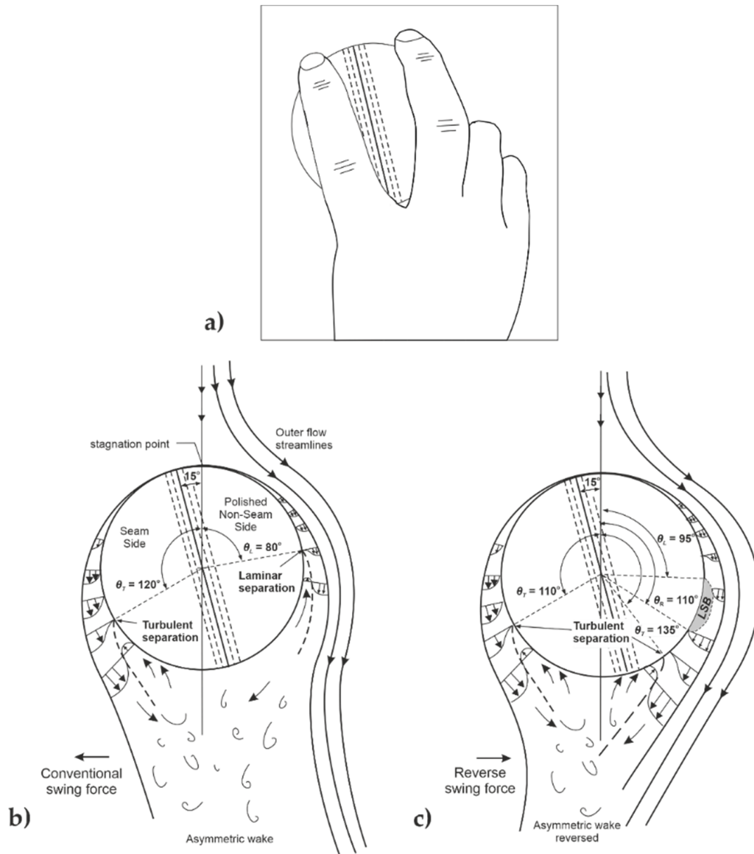
Figure 1. (a) Illustration of a right-handed bowler’s grip on a cricket ball for swing; (b) conventional swing, i.e., away-swing to right-handed batsman (RHB) and (c) reverse swing, i.e., in-swing to RHB. The laminar separation bubble is highlighted by the grey in-fill.
