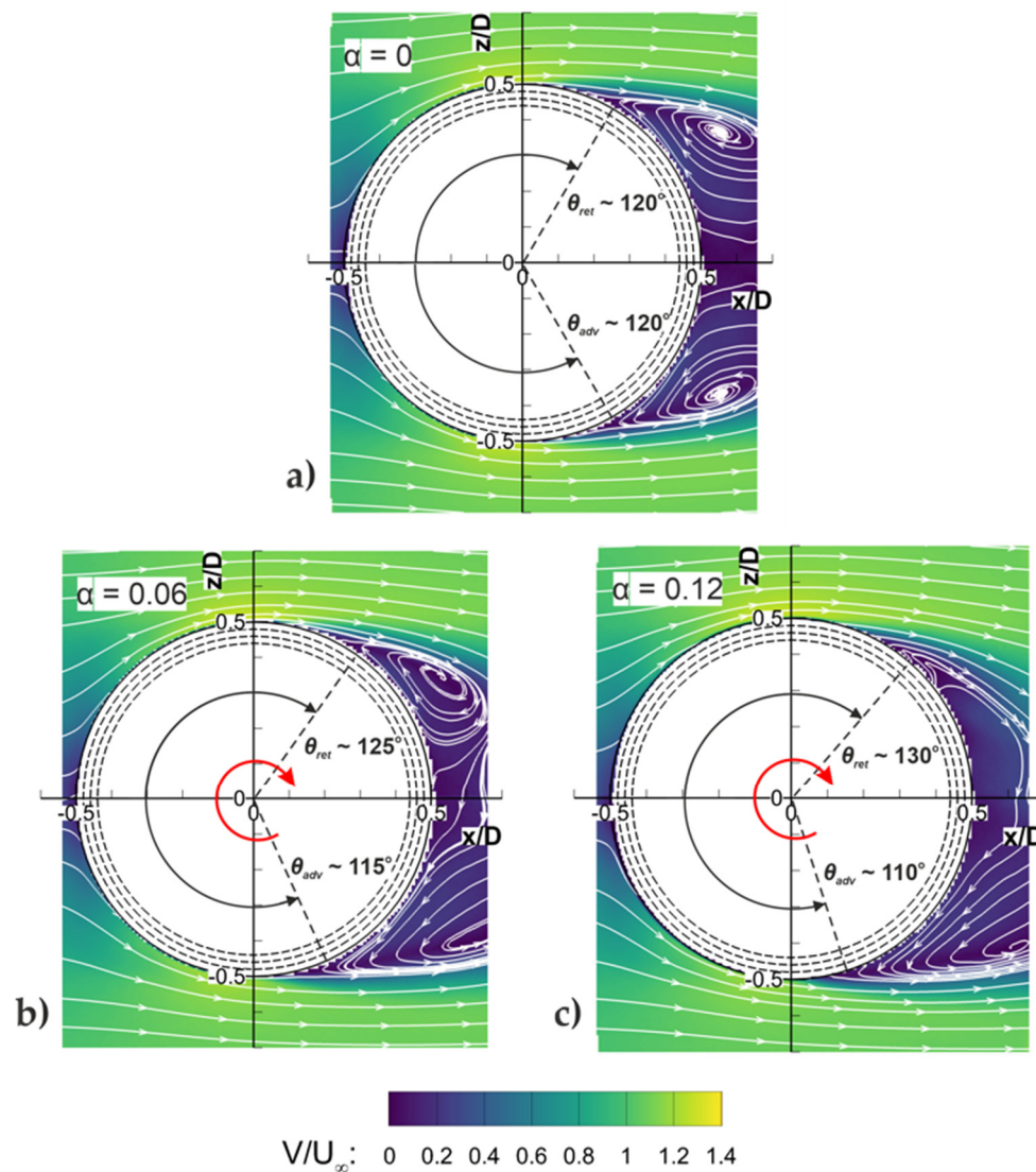
Figure 12. Time-averaged velocity magnitude in the x - z plane at Re = 1.94 \times 10^5 ( U_\infty = 20 m/s) showing (a) the symmetric flow field with no rotation and (b,c), the Magnus effect demonstrated at two different spin rates. Separation angles shown to nearest 5^\circ .
