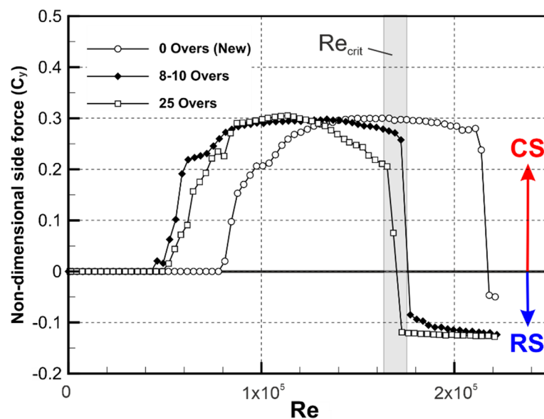
Figure 3. Variation of non-dimensional side force ( C_y ) with Reynolds number ( Re ) for Dukes balls at different stages of wear, showing the transition from CS to RS. The double-sized ball used in this paper is comparable in surface roughness to the 25-over-old ball. The critical region for the 25-over-ball is highlighted ( 1.65 \times 10^5 < Re_{crit} < 1.75 \times 10^5 ). Adapted from [4].
