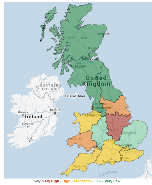
b) Snapshot of the carbon intensity of Great Britain's electricity generation. 28 Estimated values at 2020-03-09 18:30; carbon intensity groups defined by \text{gCO}_2 \cdot \text{kWh}^{-1} as Very High (360+), High (260-359), Moderate (160-259), Low (60-159) and Very Low (0-59). Basemap by GeoBasis-DE/BKG (©2009), Google, Inst. Geogr. Nacional.
