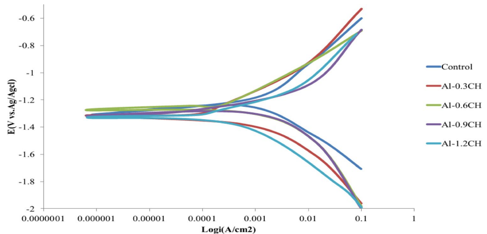
Fig. 2 Potentiodynamic polarization curves for inhibited and uninhibited aluminium alloys
