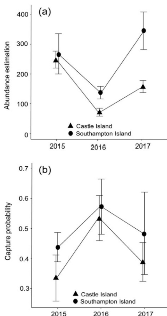
FIG. 3 (a) Comparison of M_{th} Chao robust design model of Bermuda skink abundance estimates with standard error (vertical bars) on Southampton Island and Castle Island, Bermuda, during 2015–2017. (b) Comparison of M_{th} Chao robust design model of Bermuda skink capture probability with standard error (vertical bars) on Southampton Island and Castle Island, Bermuda, during 2015–2017.
