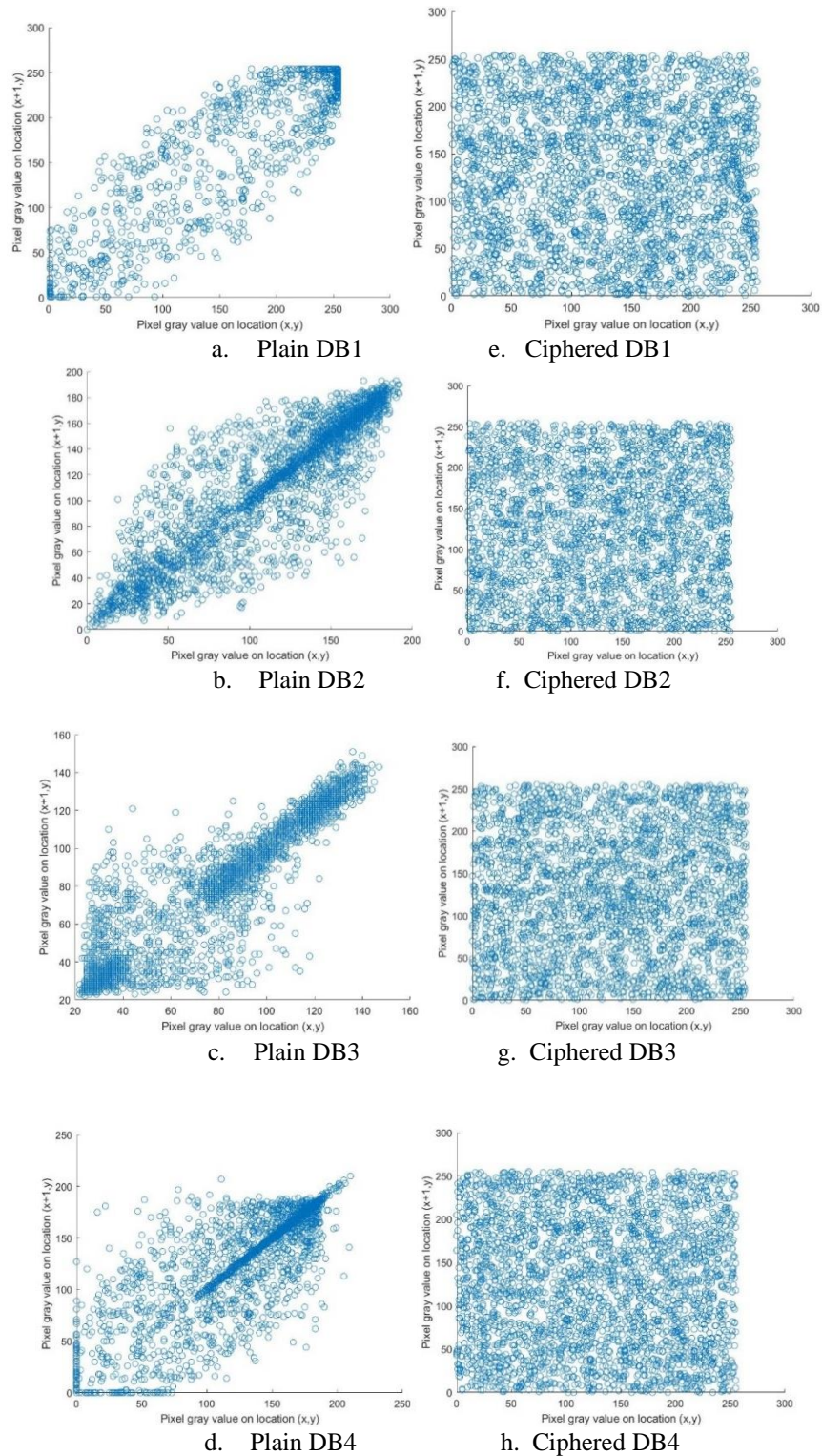
Figure 4. (a)-(d) Correlation distribution of fingerprint image for each dataset; and (e)-(h) Correlation distribution of cipher fingerprint image
