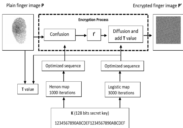
Figure 2. The proposed chaotic-based encryption process using Henon and logistic maps
