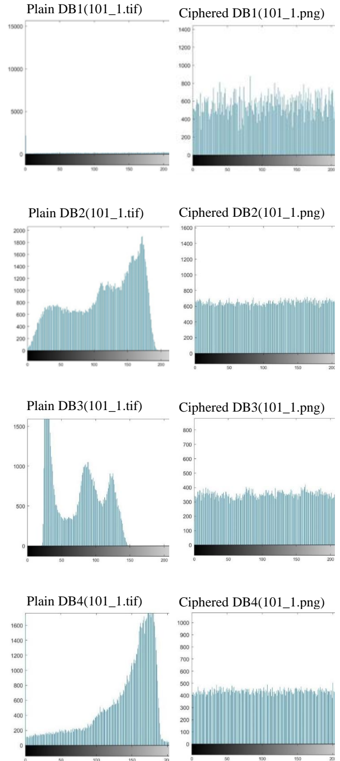
Figure 3. Histograms for the plain and ciphered fingerprint images
