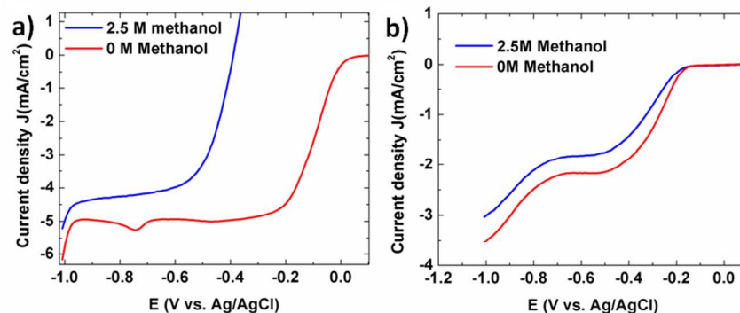
Fig. 8: (a) Polarization curves for ORR on commercial Pt/C catalyst in an O_2 -saturated 0.1 M KOH electrolyte containing 2.5 M methanol at a rotation rate of 1600 rpm and scan rate of 10 mV/s. (b) Polarization curves for ORR on ErGO electrode in an O_2 saturated 0.1 M KOH electrolyte containing 2.5 M methanol at a rotation rate of 1600 rpm and scan rate of 10 mV/s.
