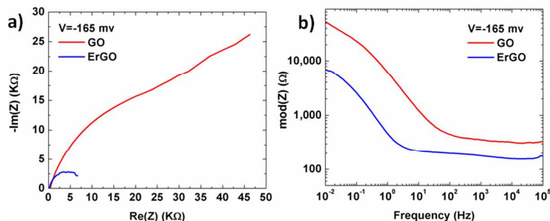
Fig. 9: (a) Nyquist plots and (b) Bode plots of GO and ErGO obtained at a bias of -0.165 V over the frequency range from 100 kHz to 10 mHz.
