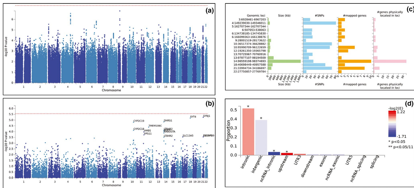
Figure 2 Association results from analyses adjusted by age, sex, PCs and CYP2C19 *2 variant (a) Single-nucleotide polymorphism (SNP)-based genomewide association study (GWAS) Manhattan plot where chromosome position is on x-axis and -\log_{10} of association P value on y-axis (genomic inflation factor = 1.01). (b) Gene-based GWAS Manhattan plot of performed by MAGMA highlighting top 15 genes. (c) Summary of lead SNPs identified by the analyses; (d) functional annotation of lead SNPs and SNPs in linkage disequilibrium (LD) using ANNOVAR.
