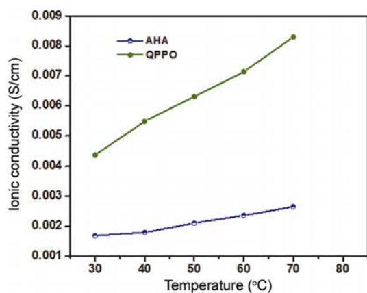
Figure 3. Conductivity for QPPO and AHA membranes as a function of temperature.
