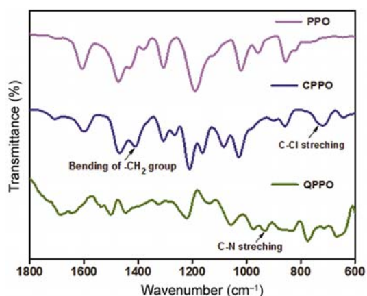
Figure 2. FT-IR spectra of PPO, CPPO and quaternized PPO.
