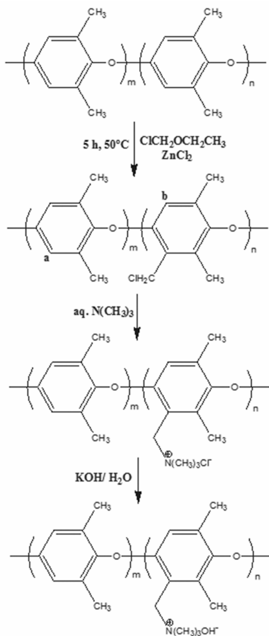
Scheme 1. Synthetic procedure for preparation of quaternized PPO membrane.
