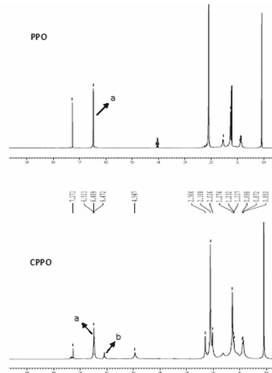
Figure 1. ^1\text{H} NMR spectra of PPO and CPPO.
