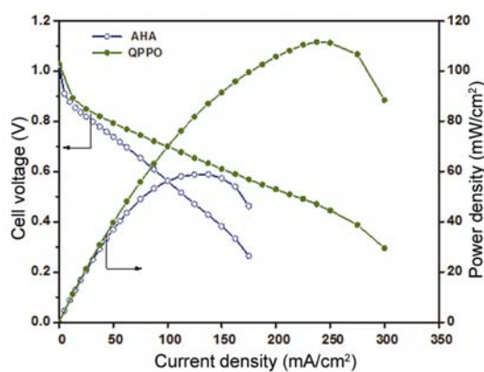
Figure 4. Cell performance curves of APEFCs comprising AHA and QPPO membranes.
