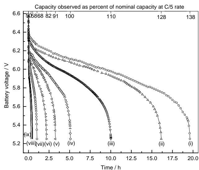
Figure 7. Performance characteristics of a 6 V/3.5 Ah lead-acid battery with lightweight modified grids obtained at 25°C for (i) C/20, (ii) C/15, (iii) C/10, (iv) C/5, (v) C/3, (vi) C/2, (vii) C, (viii) 2C, and (ix) 3C discharge rates.
