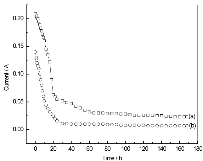
Figure 5. Comparative potentiostatic corrosion data for (a) ABS/Cu/Pb, and (b) ABS/Cu/Pb/PANI positive grids at a charging voltage of 2.5 V at 55°C.
