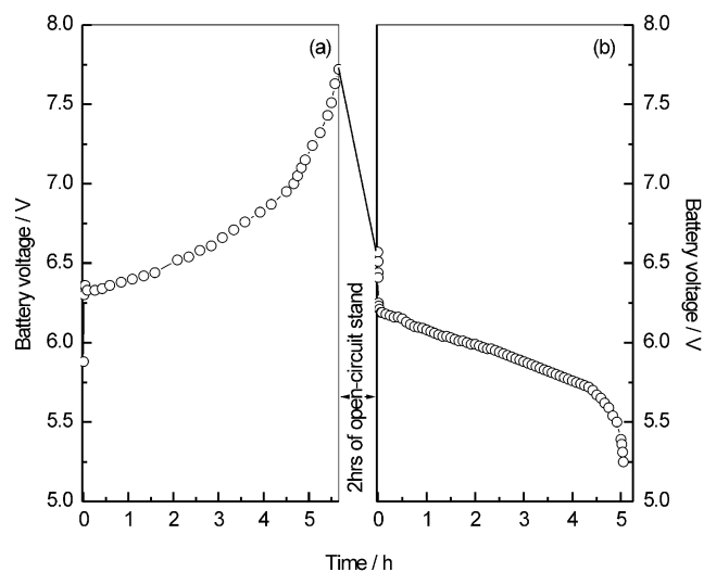
Figure 6. A typical C/5 rate galvanostatic charge-discharge data for a 6 V/3.5 Ah lead-acid battery with lightweight modified grids obtained at 25°C.
