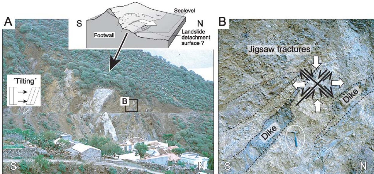
Fig. 4 Photographs of sheared northern sector of Anaga. Landslide detachment surface is eroded and thus not found near sea level (see inset). (A) The footwall is intensely sheared, movement “top to the north”. Dikes of the oldest WSW-ENE rift zone show intrusive volumes reaching up to \sim 90\% of the rock mass. (B) Close-up photo illustrates mixed-mode shearing and jigsaw fractures. Dike intrusions here occurred prior to fracturing. The material is extremely altered and unstable. Strong shearing and fragmentation has led to structures resembling those of proximal debris avalanche deposits. Dike traces are unclear and have diffuse margins, a feature that earned them the name “ghost dikes” by local geologists (Spanish “diques fantasma”)
