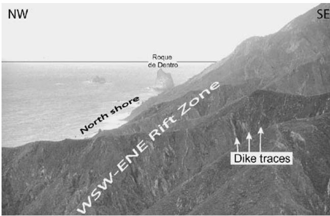
Fig. 3 Taganana embayment looking eastward (photograph taken north of the El Bailadero tunnel, see Fig. 2a). Most rocks here are dikes, inclined to the south (to the right of the picture). Later dikes (arrows) have wavy contacts and intruded subvertically
