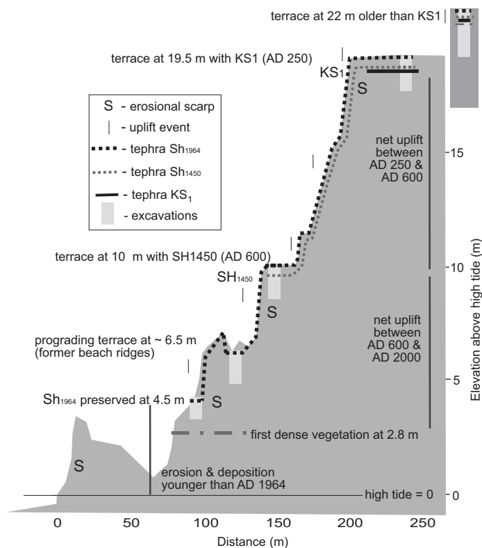
Figure 4. An example of a profile (profile 23) with very rapid net uplift. The profile is made of steep steps; steeper faces indicate cliff retreat and erosion. Tephtras KS_1 , SH_{1450} , and SH_{1964} are interpreted to be truncated by erosion, rather than pinching out (see Figs. 5 and 6). Additional profiles are shown in Figure DR1 (see text footnote 1).
