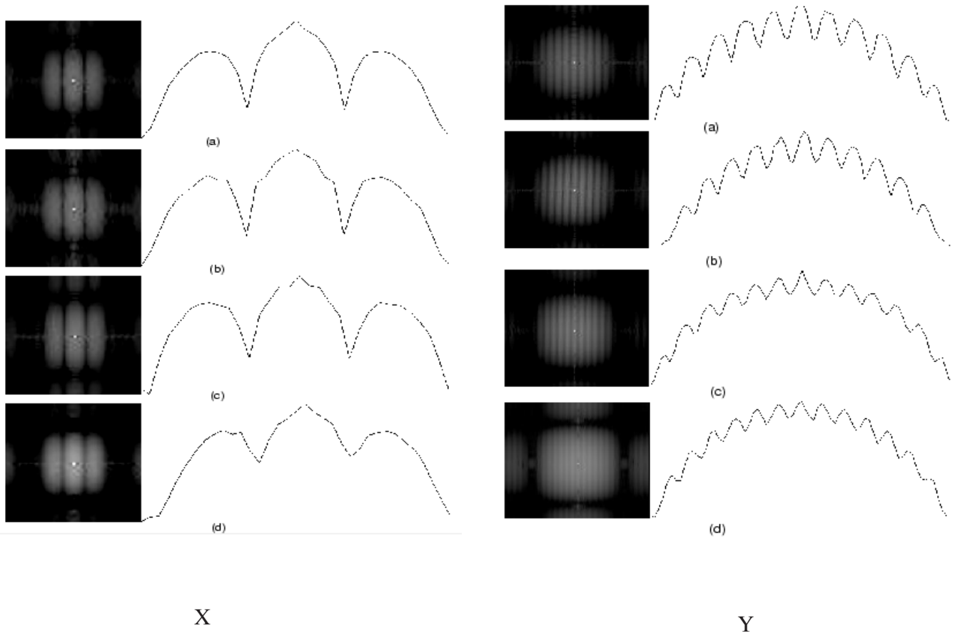
Fig. 2—Interference fringes and relative intensity distribution of specimens [(a) Ra = 1.57 μm; (b) Ra = 3.1 μm; (c) Ra = 4.5 μm; (d) Ra = 6.25μm] at displacement: X) 20 μm; Y) 100 μm
