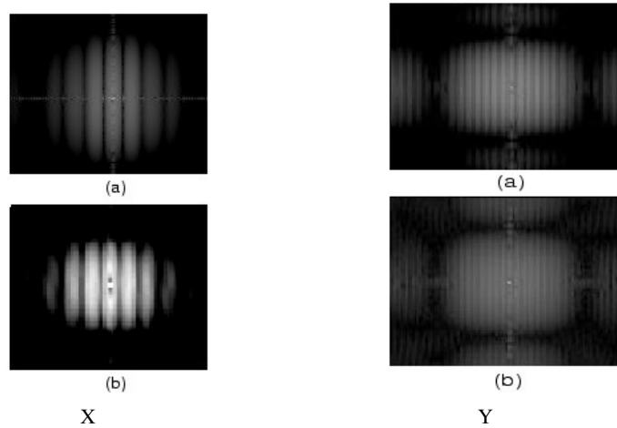
Fig. 5—Young’s fringes for surfaces of Ra [(a) 1.6µm, (b) 3.17µm] at: X) \delta\theta=0.5^\circ ; Y) \delta\theta=1.5^\circ
