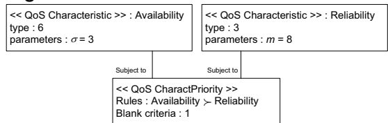
Figure 3. Instantiation of the QoS metamodel
