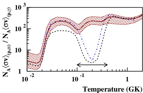
FIG. 4: Ratio of the ^{17}\text{O}(p,\alpha)^{14}\text{N} and ^{17}\text{O}(p,\gamma)^{18}\text{F} reaction rates (solid line with hatched area reflecting uncertainties), in comparison with the previous results of Angulo et al. [8] (dashed line) and Fox et al. [5] (dotted-dashed line). The horizontal arrow shows the range of typical novae temperatures.
