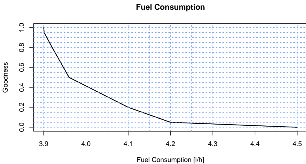
Figure 8.17: Fuzzy set to match a fuel consumption of 3.9 l/h
