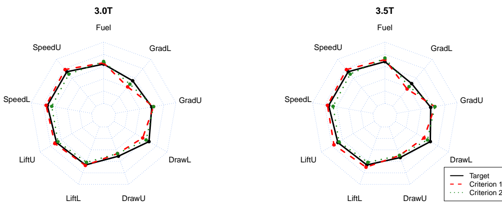
Figure 8.20: Targets vs achieved for 3T & 3.5T
