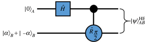
Figure 2. A quantum circuit which could be used to prepare the initial hybrid entangled states ( |\Psi\rangle_{AB}^{\text{HE}} and |\Psi\rangle_{CD}^{\text{HE}} , as given in equation (2.3)) for our proposed entanglement swapping protocol, using a Hadamard gate ( \hat{H} ) and a controlled \pi/2 rotation gate ( \hat{R}_{\pi/2} ). (Online version in colour.)
