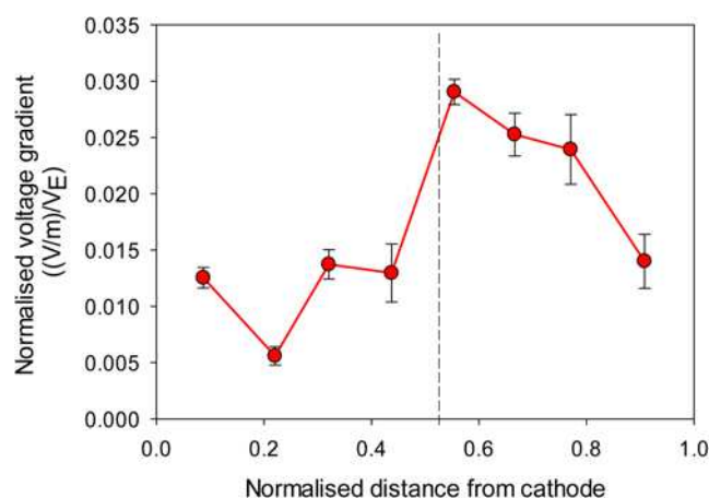
Fig. 9. Voltage gradient across the sediment section normalized to the voltage between electrodes ( V_E ) for Rig D. Error bars represent one standard deviation from the mean of four time points after the baseline. Dashed line indicates the location of the high- K –low- K interface.
