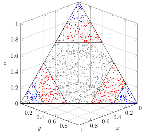
Fig. 1. The output of 1000 runs of UUnifast(3, 1).
