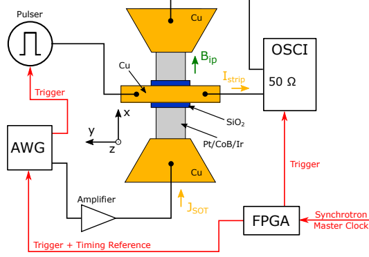
Figure 2. Schematic overview of the Pt/CoB/Ir microwire sample employed for the time-resolved measurement of the canting induced by the FL-torque and of the electrical setup used for the pump-probe experiments. The timing and synchronization signals are marked in red. J_{\text{SOT}} marks the path of the current pulse employed to generate the SOTs, and I_{\text{strip}} marks the path of the current pulse employed for the generation of the two opposite PMA domains in the Pt/CoB/Ir microwire. The direction of the applied in-plane magnetic field is indicated by the green arrow in the figure, and the coordinate system employed here is also marked in the figure.
