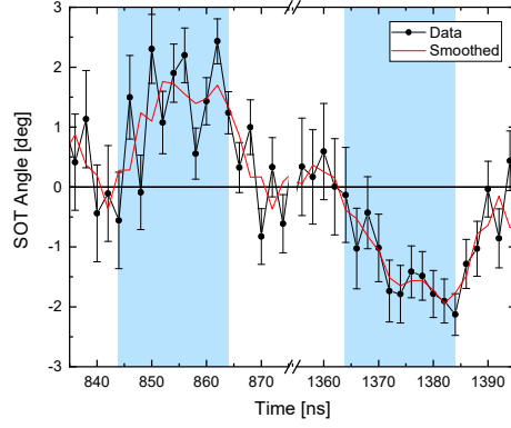
Figure 5. Calculated value of the canting angle induced by the FL-torque on the Pt/CoB/Ir microwire. A canting angle of about 1.5^\circ can be observed, and a change in its sign can be observed when applying a pulse of opposite polarity. The time steps where the pulses are applied are marked by the light blue background. The red curve shows the time trace after a 3-point adjacent average smoothing.
