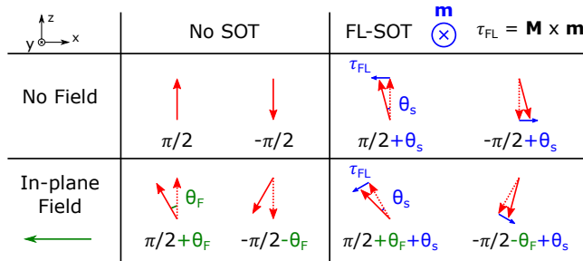
Figure 1. Schematic overview of the effect of the FL-torque on the spins in a continuous PMA domain in absence and presence of an in-plane magnetic field. In absence of both in-plane field and FL-torque, the spins in the PMA domains point either up or down (angle of \pm\pi/2 with respect to the surface plane). If the FL-torque (direction marked by the blue arrows) is applied, the two macrospins will cant of an angle \theta_S , causing an equal reduction of the M_z component for the two macrospins. However, if an in-plane magnetic field is added, the spins will cant of an angle \theta_F along the direction of the applied in-plane magnetic field (marked by the green arrow). The sign of this additional angle will depend on the original orientation of the spins. Therefore, if the FL-torque is now applied, the M_z component of the two macrospins will now be different, allowing for the extraction of the canting angle \theta_S due to the FL-torque.
