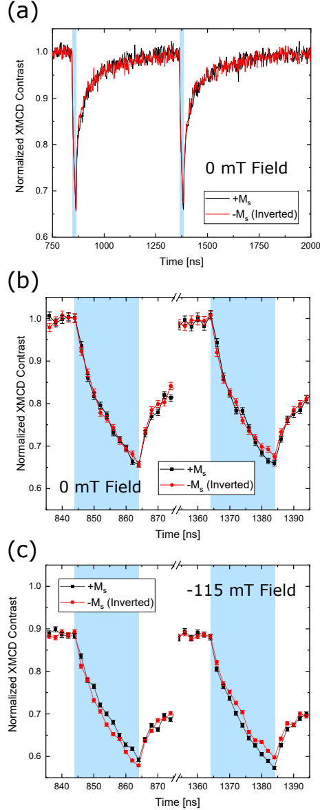
Figure 4. Time-resolved variation of the absolute value of the z component of the magnetization in the two PMA domains. The time steps where the pulses are applied are marked by the light blue background. (a) Time trace of the z component of the magnetization showing the injection of the positive and negative current pulses across the Pt/CoB/Ir microwire. A strong contribution to the dynamics of the z component of the magnetization is given by the heating caused by the injection of the current pulse. (b) Detail of (a), showing the regions where the current pulses are applied. No substantial differences can be spotted for the two PMA domains when no in-plane field is applied. (c) Time trace of the z component of the magnetization with an in-plane field of -115 mT applied. Here, a difference between the two PMA domains, attributed to the contribution of the FL-torque can be spotted.
