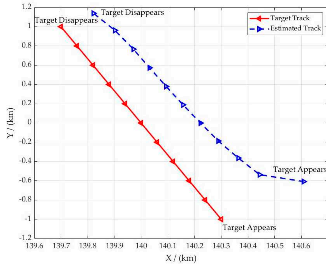
Figure 10. Target detection results by the modified ICMB filter.
