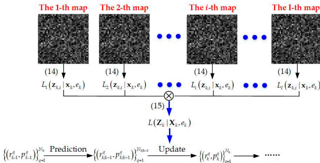
Figure 4. Propagation track table of the product multi-Bernoulli filter.
