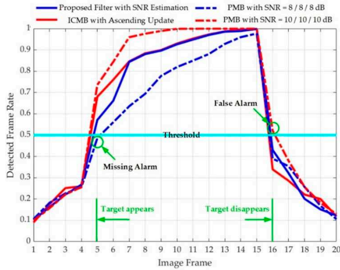
Figure 13. Comparison results of detected frame rate.
