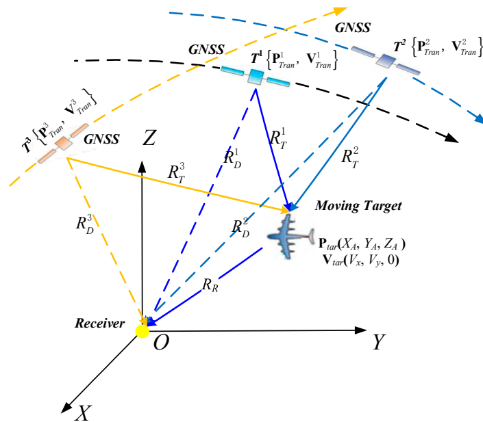
Figure 1. General geometric configuration of a multi-static global navigation satellite system based passive radar (MsGBPR) system.
