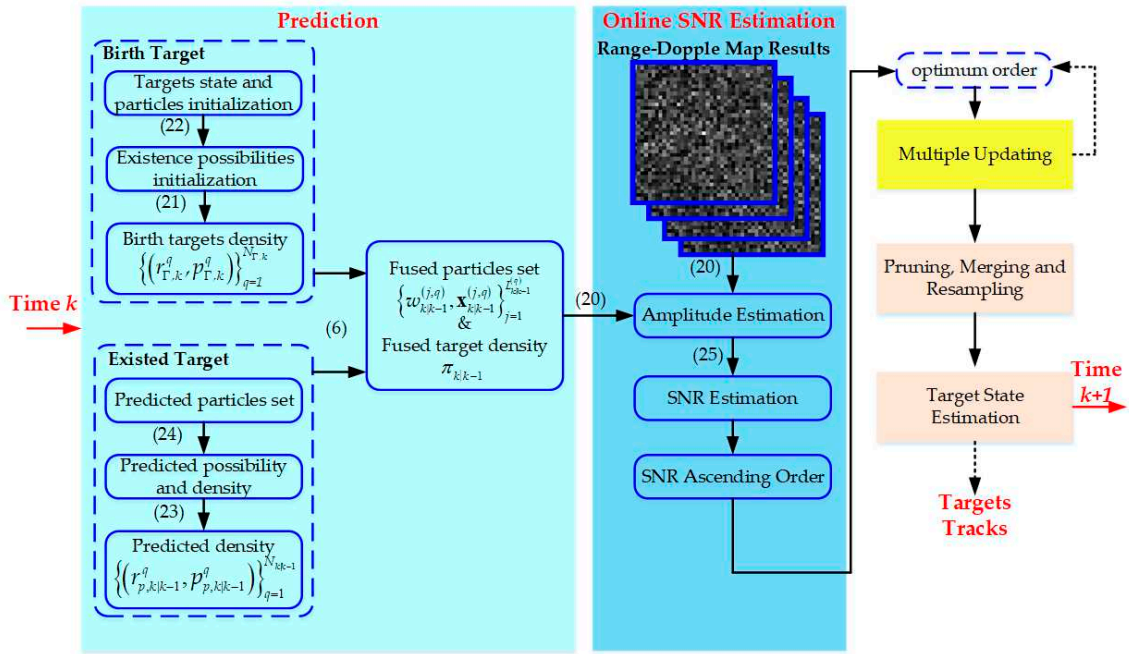
Figure 6. Sequential Monte Carlo (SMC) implementation of the proposed modified ICMB filter.
