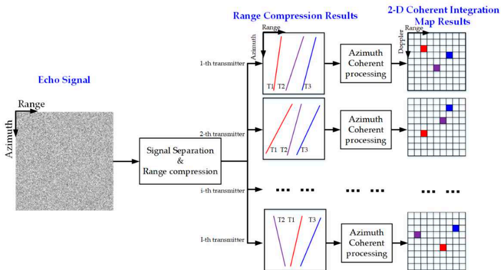
Figure 2. Diagrammatic sketch of 2-D coherent integration processing and map results in MsGBPR.
