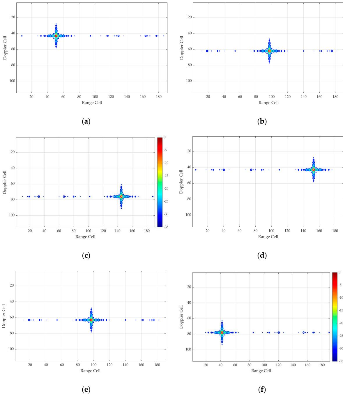
Figure 8. Noise-free range-Doppler maps results: (a–c) maps at frame-5, frame-10, and frame-15 with SVN#2 used; (d–f) maps at frame-5, frame-10, and frame-15 with SVN#10 used.
