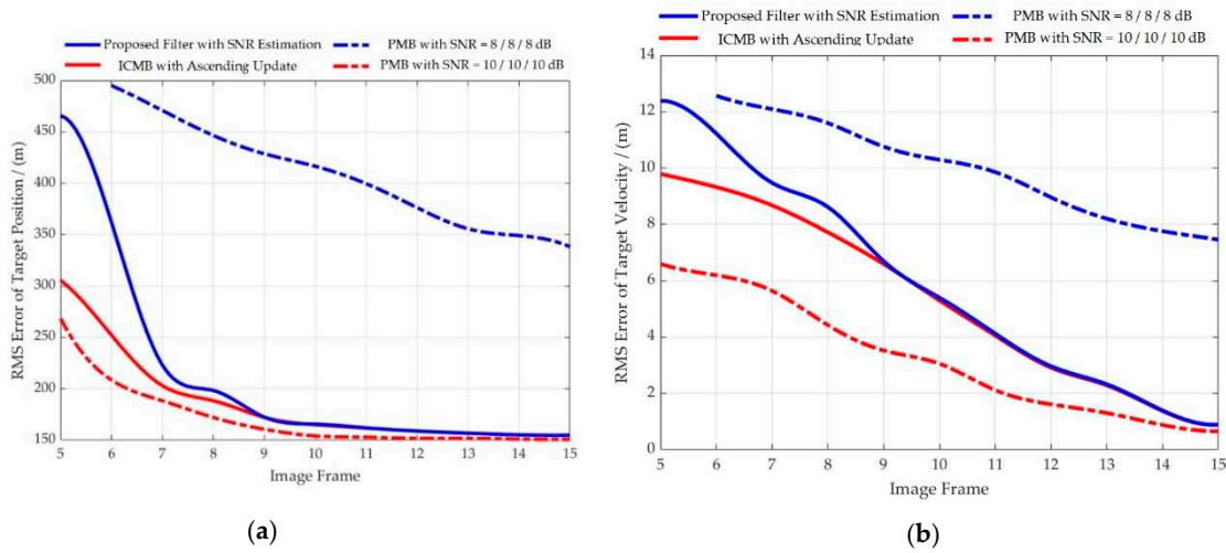
Figure 14. Comparison results of RMS errors: (a) RMS error of position; (b) RMS error of velocity.
