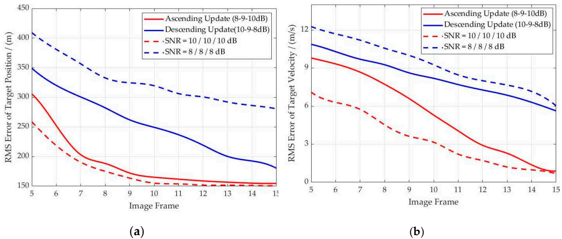
Figure 12. Root mean square (RMS) error of target position and velocity in different update order cases: (a) RMS error of target position; (b) RMS error of target velocity.
