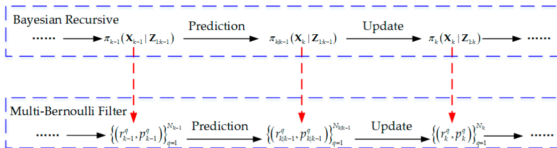
Figure 3. Propagation track table in Bayesian recursive and multi-Bernoulli filter.
