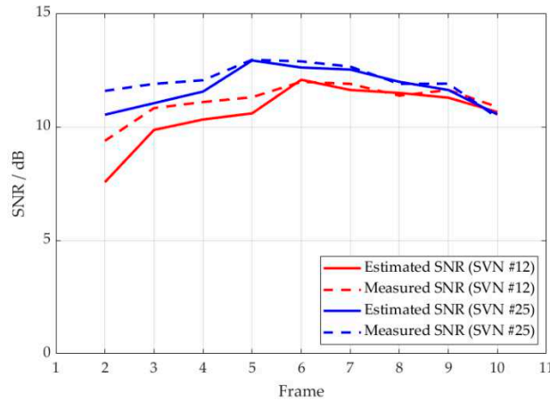
Figure 17. The estimated SNR results using the experiment data.
