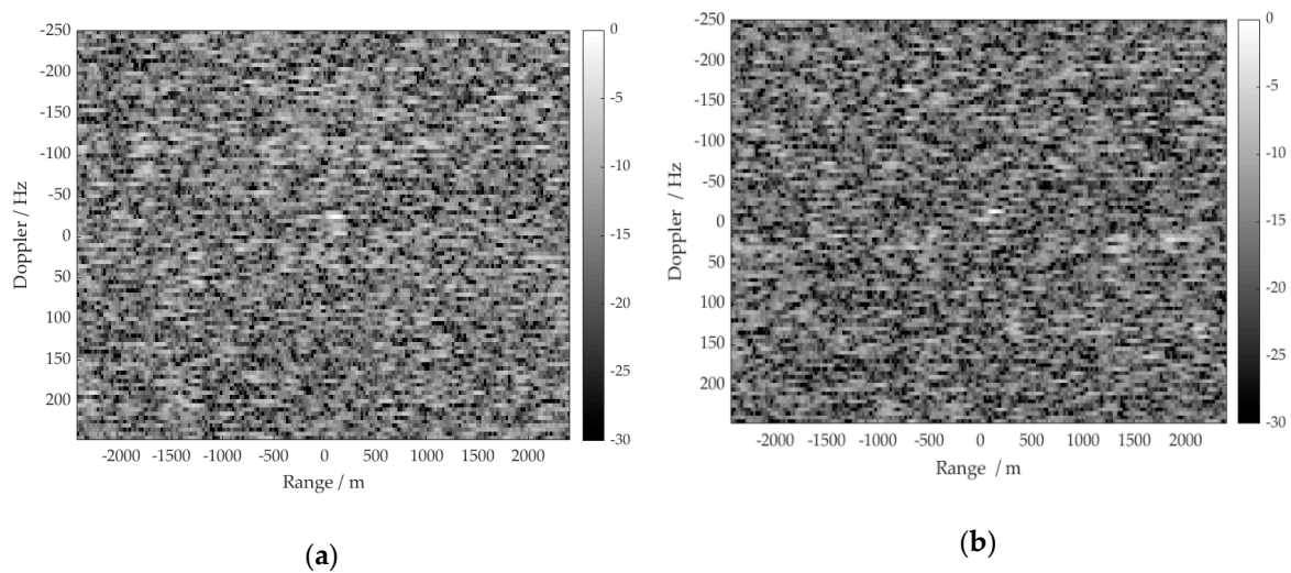
Figure 16. Experimental range-Doppler maps at frame-3: (a) SVN #12 is used as transmitter (b) SVN #25 is used as transmitter.
