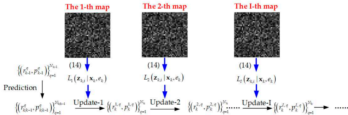
Figure 5. Propagation track table of iterated-corrector multi-Bernoulli (ICMB) filter at time k .
