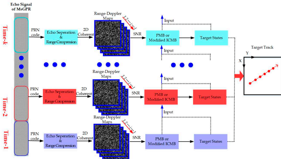
Figure 7. The proposed moving target detection framework for the MsGBPR system.
