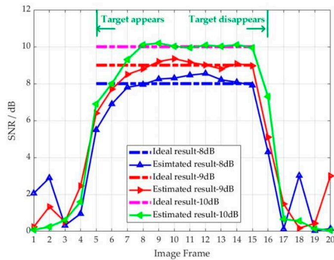
Figure 9. The online estimated signal-to-noise ratio (SNR) results for SNR_{k,i} = 8, 9, and 10 dB.
