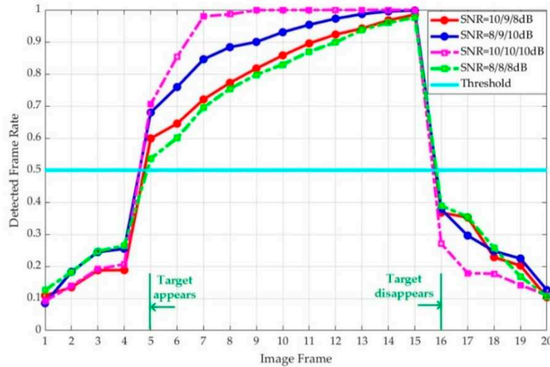
Figure 11. Detected frame rate in different update order cases.
