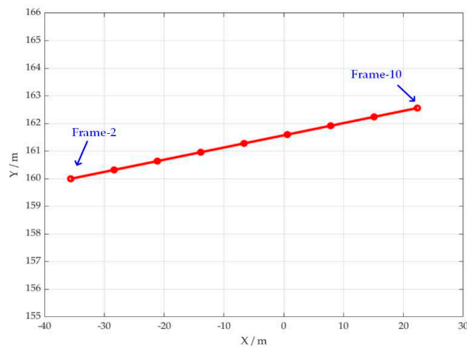
Figure 18. The estimated target track using the experiment data.
