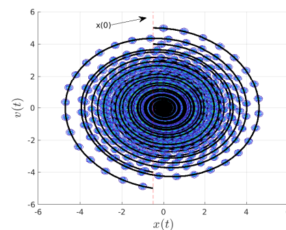
(g) Snapshots of p(x, t) for \langle x(0) \rangle = -0.5 , \gamma = 0.1 and various \langle v(0) \rangle \in (-5, 5) .
