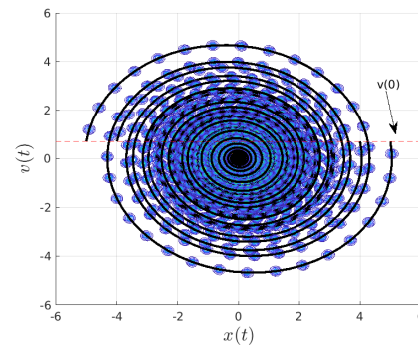
(b) Snapshots of p(x, t) for \langle v(0) \rangle = 0.7 , \gamma = 0.1 and various \langle x(0) \rangle \in (-5, 5) .
