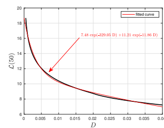
(e) \mathcal{L}_\infty = \mathcal{L}(t = 50) against D . A fitted curve is shown in the red solid line.
