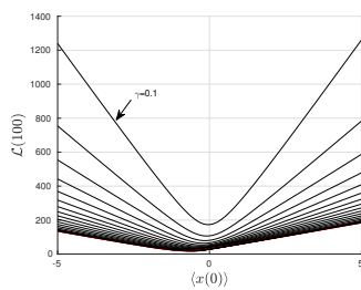
(c) \mathcal{L}_\infty = \mathcal{L}(t = 100) against \langle x(0) \rangle \in (-5, 5) for \langle v(0) \rangle = 0.7 and \gamma \in (0, 2.5) .
