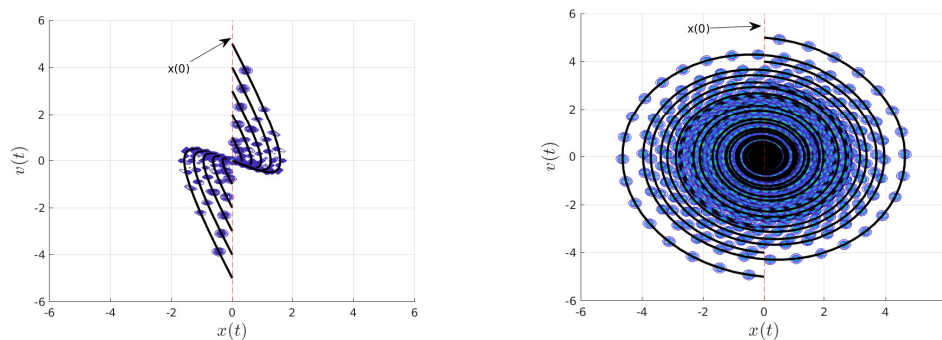
(f) Snapshots of p(x, t) for \langle x(0) \rangle = 0 , \gamma = 2.5 and various \langle v(0) \rangle \in (-5, 5) . (g) Snapshots of p(x, t) for \langle x(0) \rangle = 0 , \gamma = 0.1 and various \langle v(0) \rangle \in (-5, 5) .
