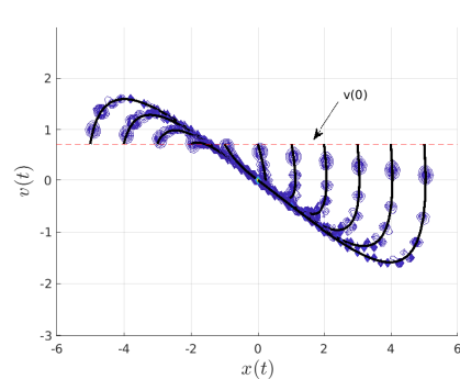
(a) Snapshots of p(x, t) for \langle v(0) \rangle = 0.7 , \gamma = 2.5 and various \langle x(0) \rangle \in (-5, 5) .
