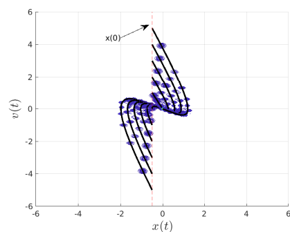
(f) Snapshots of p(x, t) for \langle x(0) \rangle = -0.5 , \gamma = 2.5 and various \langle v(0) \rangle \in (-5, 5) .
