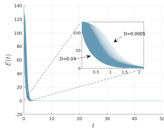
(c) Time-evolution of \mathcal{E}(t) .
