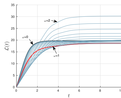
(e) Information Length \mathcal{L}(t) .
