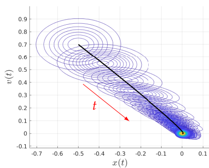
(a) Snapshots of p(\mathbf{x}, t) for D = 0.0005 .
