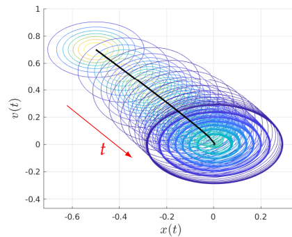
(b) Snapshots of p(\mathbf{x}, t) for D = 0.04 .
