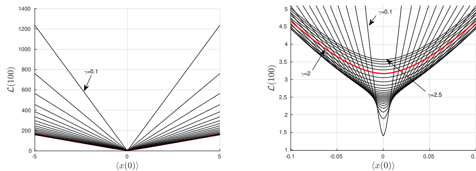
(d) \mathcal{L}_\infty = \mathcal{L}(t = 100) against \langle x(0) \rangle \in (-5, 5) for \langle v(0) \rangle = 0 and \gamma \in (0, 2.5) . (e) Zoom-in of panel (d).
