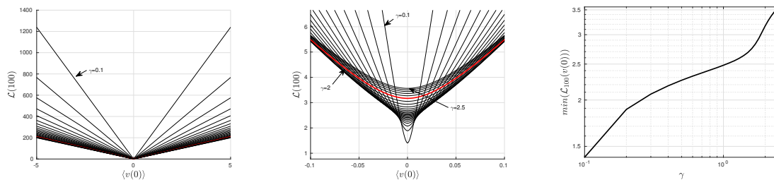
(h) \mathcal{L}_\infty = \mathcal{L}(t = 100) against \langle v(0) \rangle \in (-5, 5) for \langle x(0) \rangle = 0 and \gamma \in (0, 2.5) . (i) Zoom-in of panel (h). (j) The minimum value of \mathcal{L}_\infty against \langle x(0) \rangle = \langle v(0) \rangle = 0 against \gamma on log-log scales; \langle x(0) \rangle = 0 .
