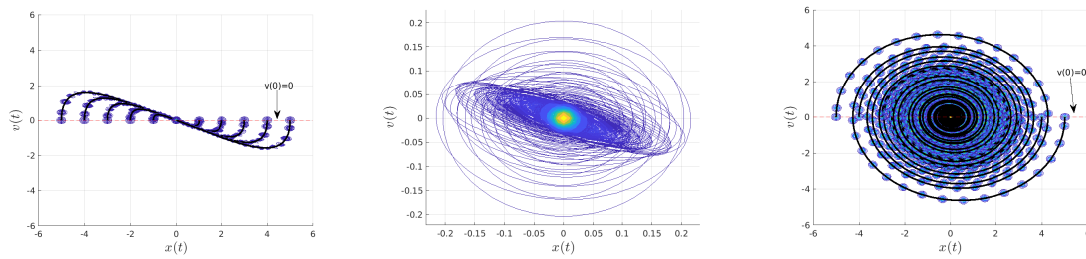
(a) Snapshots of p(x, t) for \langle v(0) \rangle = 0 , \gamma = 2.5 and various \langle x(0) \rangle \in (-5, 5) . (b) Zoom-in of panel (a) showing p(x, t) for \langle v(0) \rangle = 0 , \gamma = 2.5 and \langle x(0) \rangle = 0 . (c) Snapshots of p(x, t) for \langle v(0) \rangle = 0 , \gamma = 0.1 and various \langle x(0) \rangle \in (-5, 5) .
