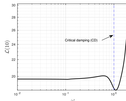
(g) The same as panel (f) but shown on log-linear scales on x - y axes.
