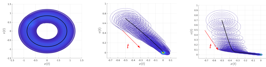
(a) Snapshots of p(x, t) for \gamma = 0 . (b) Snapshots of p(x, t) for \gamma = 2 . (c) Snapshots of p(x, t) for \gamma = 6 .
