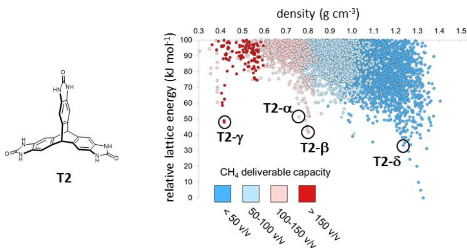
Figure 12 Chemical diagram of benzimidazolone T2 and its energy-structure-function map, showing simulated CH 4 deliverable capacities for all predicted crystal structures. 140 Experimentally observed crystal structures are circled and labelled T2-α to T2-δ . The data point for each predicted crystal
