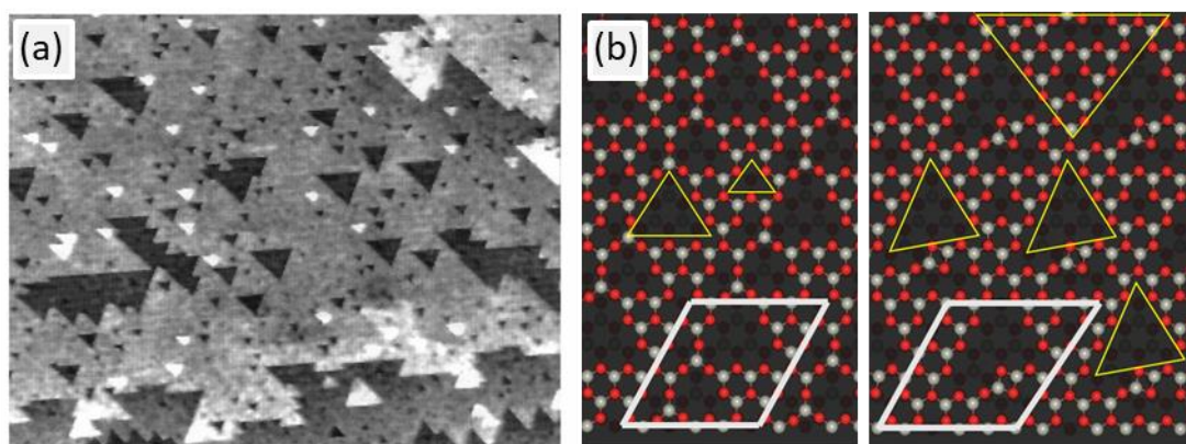
Figure 6 Left: SEM Image of the (0001) Zn terminated surface of ZnO after Parker et al. 107 (Reprinted from Surface Science , Vol 415, T.M.Parker, N.G.Condon, R.Lindsay, F.M.Leibslle, G.Thornton, Imaging the polar (000 \bar{1} ) and non-polar (10 \bar{1}0 ) surfaces of ZnO with STM, p L1046-L1050, Copyright (1998), with permission from Elsevier); Right: Two predicted low energy configurations of the reconstructed Zn terminated polar surface of ZnO, after Mora Fonz et al. 108 The white and yellow lines indicate the unit cell and observed triangular patterns, respectively.
