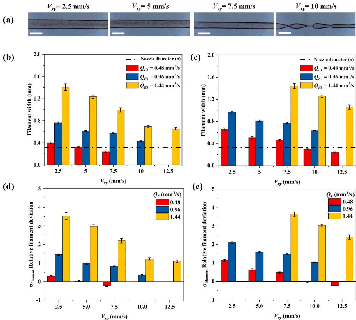
Fig. 5. Printed filament width of D\_PCL/PEO changes with various print speed V_{xy} when the extrusion rate Q_E = 0.48 \text{ mm}^3/\text{s} , the scale bar is 500 \mu\text{m} (a); the DIW printed filament width of D\_PCL/PEO (b) and A\_PCL/PEO (c) and the relative filament deviation ( \sigma_{\text{filament}} ) of D\_PCL/PEO (d) and A\_PCL/PEO (e) under the designated printing speed and extrusion rate.
