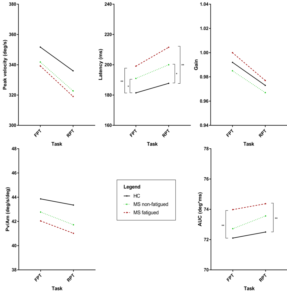
Fig 2 Saccadic parameters of healthy controls, fatigued and non-fatigued MS patients
