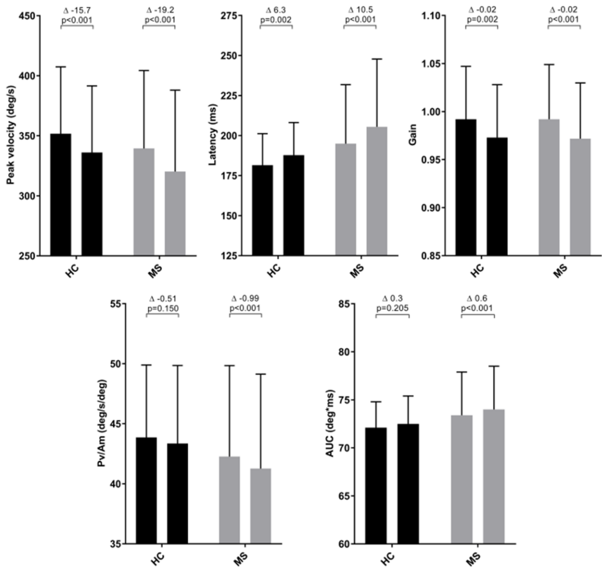
Fig 1 Saccadic parameters of healthy controls and MS patients
