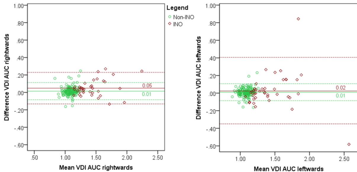
Fig 3 Bland-Altman plots of the VDI AUC
