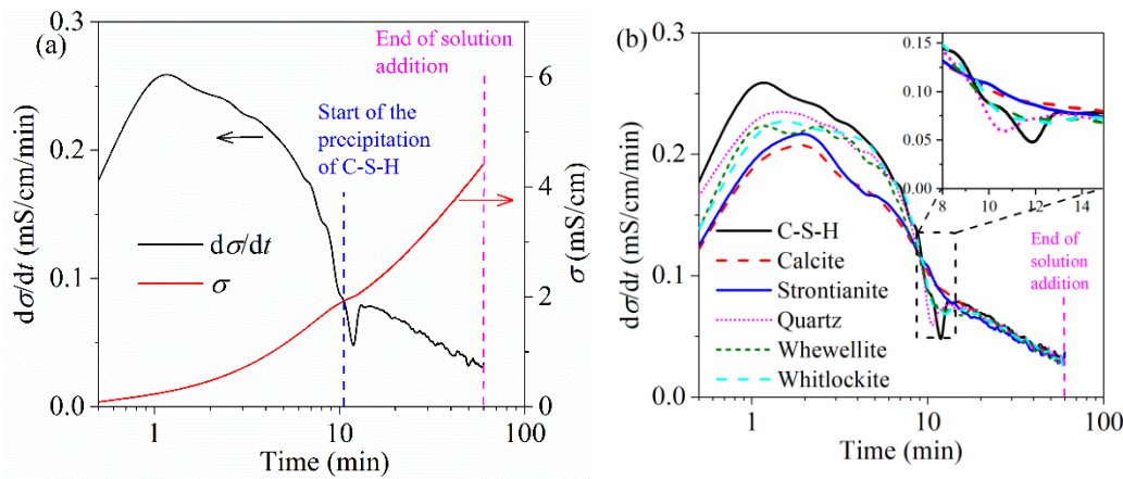
Fig. 7 The electrical conductivity of the solution. (a) The electrical conductivity of the solution without fillers (red line) and its differential curve (black line); (b) The differential electrical conductivities of solutions with or without fillers.
