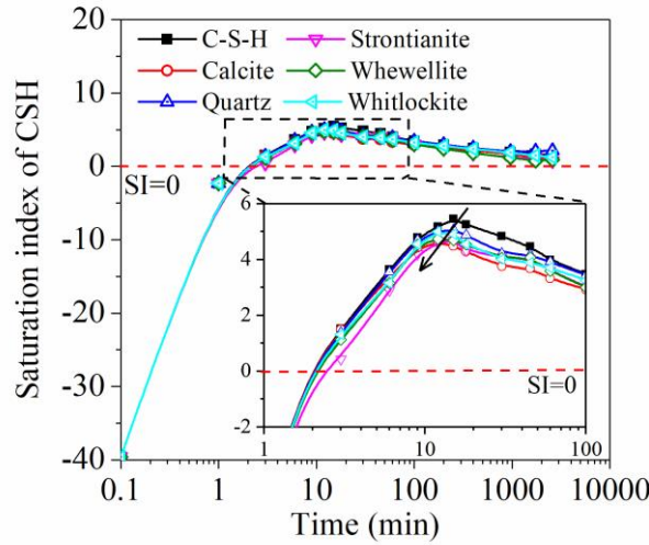
Fig. 9 Saturation index of C-S-H (CSH_T5C, Ca/Si=1.0) in different systems.
