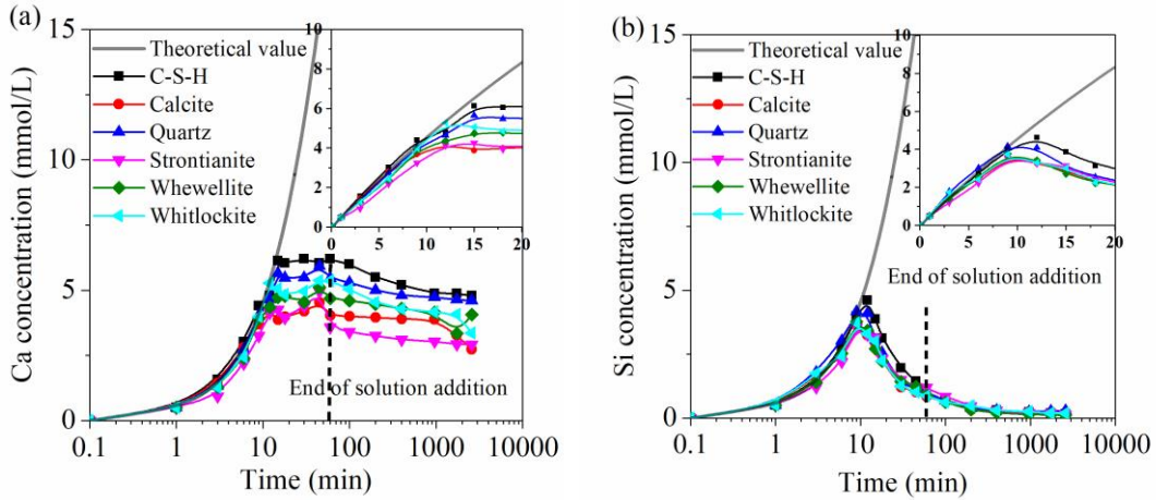
Fig. 8 Ion concentrations of the solutions. (a) Ca concentration decreases slowly after the precipitation of C-S-H; (b) Si concentration decreases rapidly after the precipitation of C-S-H.
