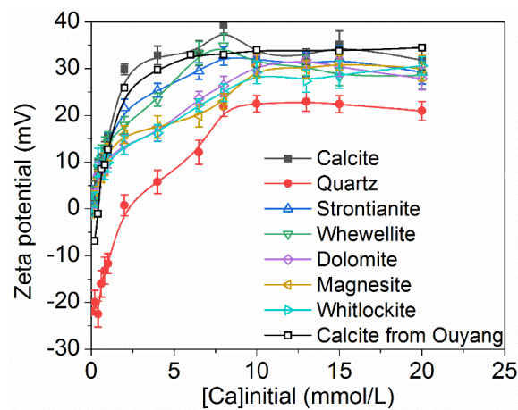
Fig. 4 Zeta potentials of the filler suspensions as a function of the initial calcium concentrations. Hollow box data are the zeta potentials of calcite suspensions adopted from Ouyang et al. [8, 12]
