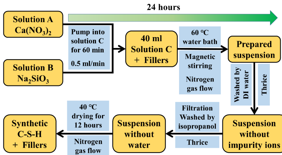
Fig. 1 Schematic diagram of the synthetic procedure of C-S-H with fillers.
