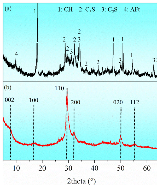
Fig. 2 XRD patterns. (a) OPC paste at 360 days; (b) synthetic C-S-H without fillers.
