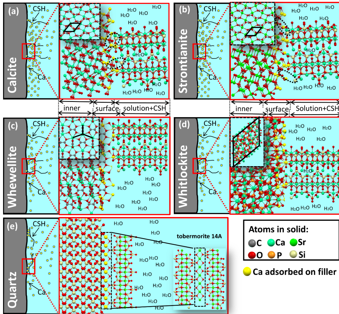
Fig. 10 Schematic diagram of the nucleation and growth of synthetic C-S-H on different fillers. (a) C-S-H on calcite; (b) C-S-H on strontianite; (c) C-S-H on whewellite; (d) C-S-H on whitlockite; (e) C-S-H on quartz.
