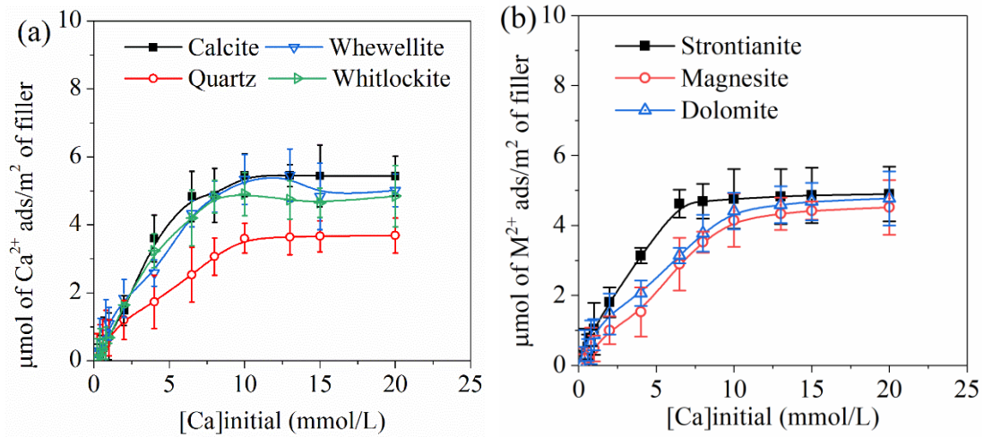
Fig. 3 Content of Ca^{2+} adsorbed on the unit surface area of fillers. (a) Adsorption of Ca^{2+} on the surface of fillers without ion exchange; (b) total adsorption of cations ( Ca^{2+} , Sr^{2+} and Mg^{2+} ) on the surface of fillers with ion exchange.
