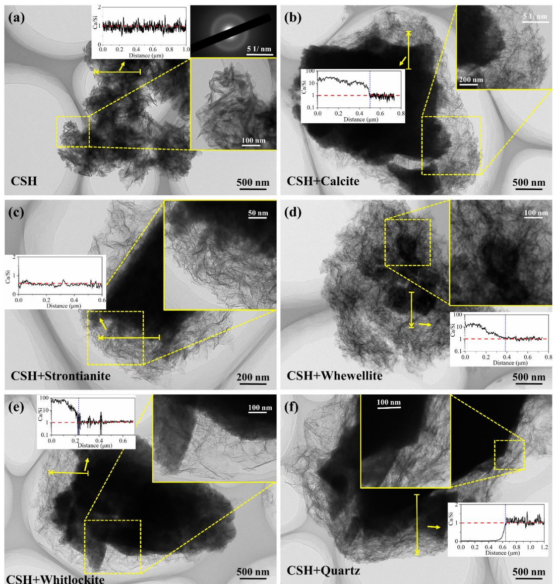
Fig. 6 TEM morphology of synthetic C-S-H on fillers. (a) Pure C-S-H; (b) C-S-H on calcite; (c) C-S-H on strontianite; (d) C-S-H on whewellite; (e) C-S-H on whitlockite; (f) C-S-H on quartz. The Ca/Si ratio of C-S-H on strontianite is approximately 0.7, while those of the other C-S-H are approximately 1.0. (what are the
