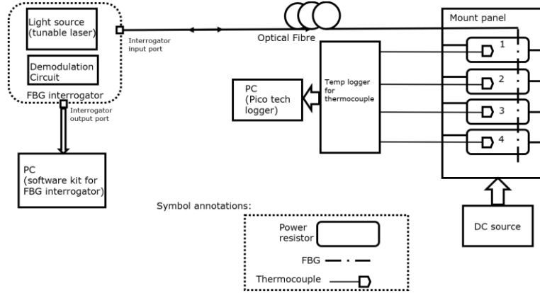
Figure 1 A prototype simulating EM windings for hot-spots temperature measurement
