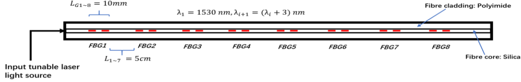
Figure 2 Structure of Polyimide-coated multi-FBG string
