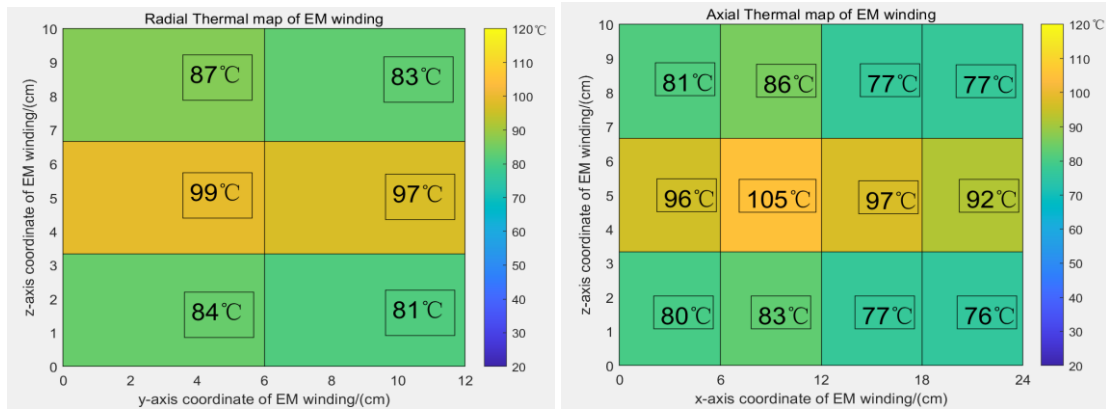
Figure 5 a) Radial thermal map (left panel), and b) axial thermal maps (right panel) of EM windings with multi-FBG string embedded prototype. The experimental parameters are shown in Figure 4.
