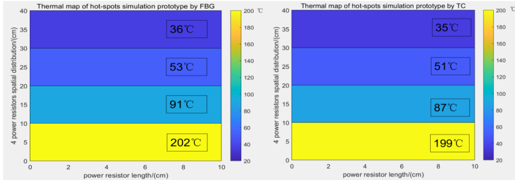
Figure 4 Thermal maps of equivalent hot-spots prototype measured by a) FBG sensors and b) thermocouples
