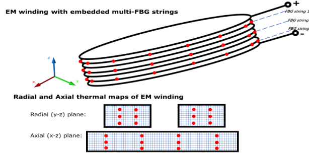
Figure 3 Schematic of three multi-FBG strings embedded together with an EM windings.
