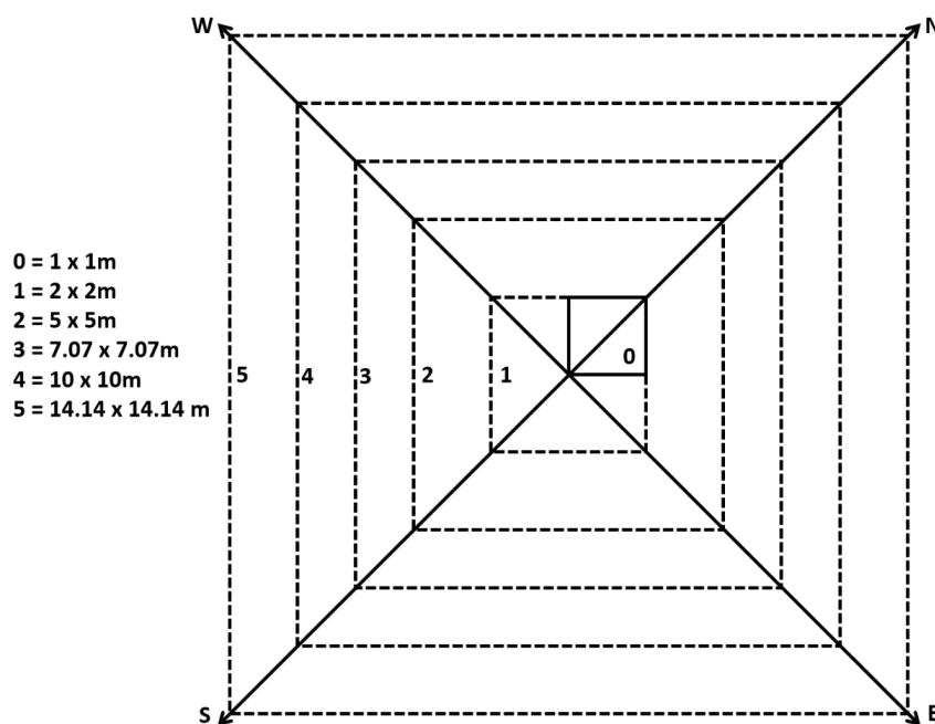
Figure 2. X-plot design for vegetation sampling [33].
