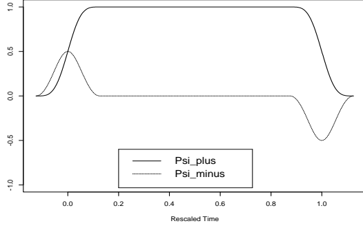
Figure 4: The bells \Psi_+ and \Psi_- .
