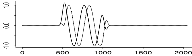
Figure 3: A SLEX waveform with support on block S(2,1) oscillating at frequency index 2.
