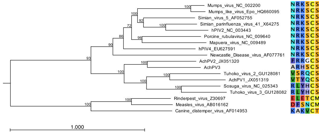
Figure 6. The phylogenetic relationship of the AchPV3 Hemagglutinin protein among other paramyxoviruses (pararubulaviruses, orthorubulaviruses, and morbilliviruses). Midpoint-rooted maximum likelihood phylogenetic tree based on a 581 amino acid alignment and the scale bar is in expected substitutions per site. Adjacent to the label names is the hexapeptide motif found in the paramyxoviral attachment proteins.
