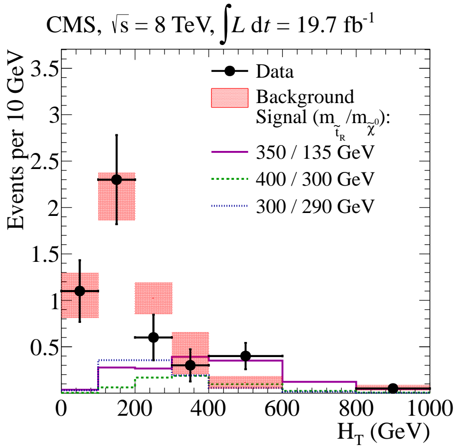
Figure 9: H_T distributions for the data, background prediction, and representative signals for the three event categories combined. The last bin includes the overflow.
